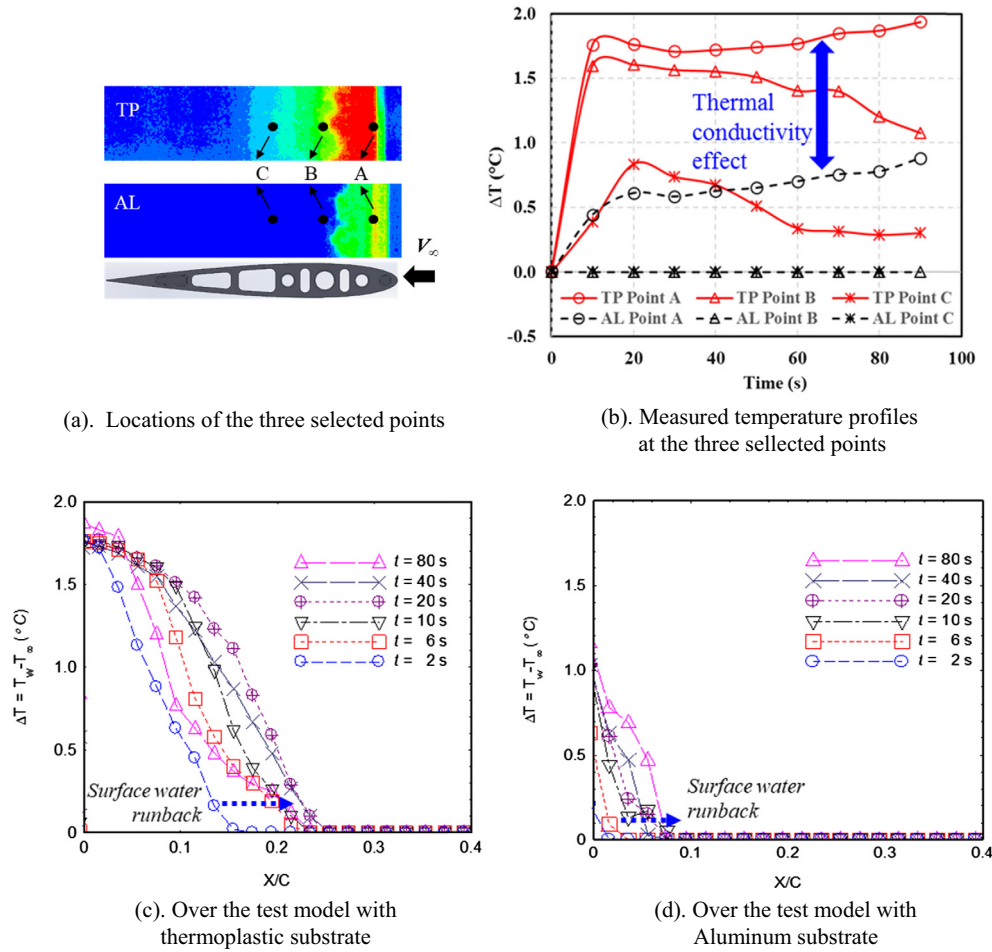
Fig. 6. Measured surface temperature profiles extracted from the IR thermal images for the test case under the glaze icing condition of V_{\infty} = 40 m/s, T_{\infty} = -5 ^{\circ}\text{C} and LWC = 2.0 g/m 3 .
