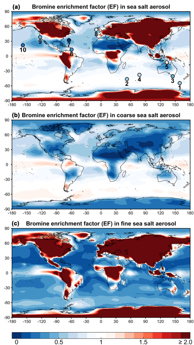
Figure 1. Annual mean bromine enrichment factor (EF) of sea salt aerosol (SSA) in surface air. GEOS-Chem model results (contours) are compared to observations (circles in a ). (a) shows results for total SSA (fine + coarse), (b) is for coarse SSA ( > 0.5 \mu\text{m} radius), and (c) is for fine SSA ( \leq 0.5 \mu\text{m} radius). Observations at 10 sites compiled by Sander et al. (2003) and from Newberg et al. (2005) are superimposed as circles and labeled in order 1–10: Macquarie Island, Crozet Islands, Cape Grim, Amsterdam Island, Jabiru, Barbados, Bermuda, Mace Head, Bodega Bay, and Hawaii, respectively. The simulation is for 2012 and the observations are for different years. Color bar saturates at 2.0. Maximum modeled EF is 75.0.
