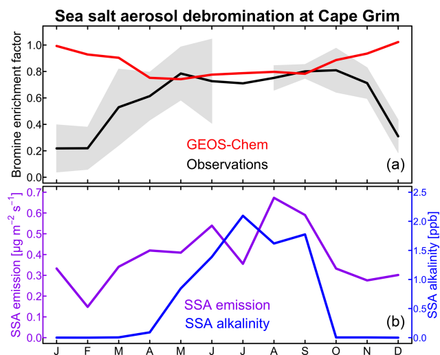
Figure 2. Seasonal variation of sea salt aerosol (SSA) debromination at Cape Grim, Tasmania ( 40.7^\circ \text{S} , 144.7^\circ \text{E} ). (a) shows the bromine enrichment factors (EFs) of monthly mean SSA in surface air. Observations from Ayers et al. (1999) and Sander et al. (2003) for 1996–1998 are compared to GEOS-Chem model values for 2012. Shading gives the interannual standard deviation in the observations. (b) shows the GEOS-Chem monthly SSA emission flux at Cape Grim (site 3 in Fig. 1) and the SSA alkalinity. The SSA emission flux is for the oceanic fraction of the Cape Grim grid square.
