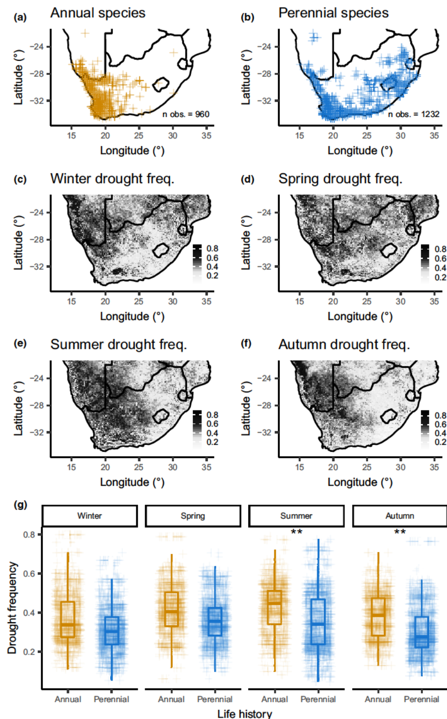
Fig. 2 Locations of occurrence records of (a) annual and (b) perennial Heliophila . Drought frequency during the (c) winter, (d) spring, (e) summer and (f) autumn detected using the Vegetative Health Index (VHI). (g) Drought frequencies during each season at the observation locations of annual and perennial Heliophila (post hoc contrasts annuals and perennials from ANOVA, **, P < 0.01 ). Boxplots indicate median (horizontal line), first and third quartiles (upper and lower limits of box), and 1.5 times the interquartile range (whiskers). Individual observations are shown by crosshairs. Annual and perennial species are indicated by data coloured blue and orange, respectively.
