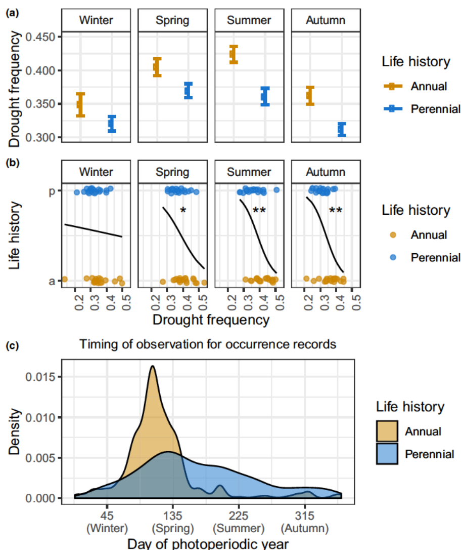
Fig. 3 Difference in drought regimens and phenology of annual and perennial Heliophila . (a) Comparison (mean \pm SE) of drought frequency across seasons calculated at the occurrence locations of GBIF records of annual and perennial species of Heliophila . (b) Results from phylogenetic logistic regression, where the line shows the model fit and *, P < 0.05 , **, P < 0.01 . Annuals were scored as 0 and perennials as 1. (c) Collection dates of GBIF records of annual and perennial species of Heliophila in relation to the photoperiodic calendar where day 1 is intermediate to the autumn equinox and winter solstice.
