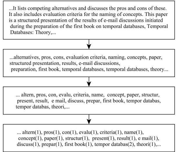
Figure 4: Preprocessing text for the machine learning step.
