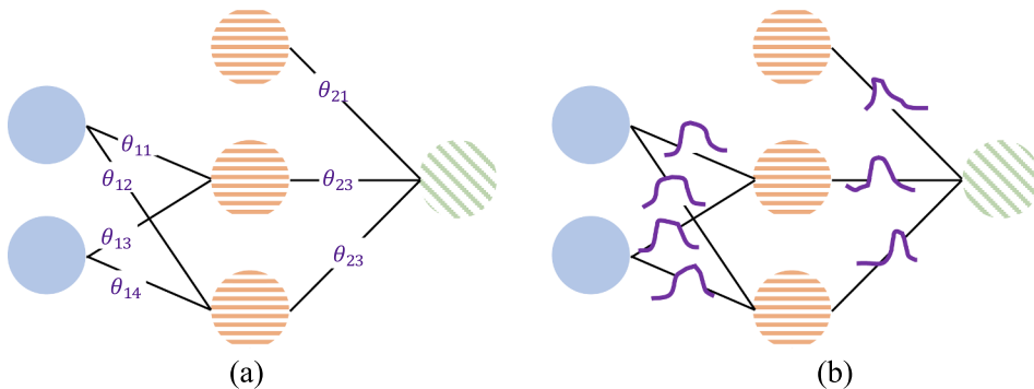
Fig. 4. Comparisons between a traditional neural network and a Bayesian neural network: (a) parameters in a traditional neural network are fixed values, (b) parameters in a Bayesian neural network are probability distributions.
