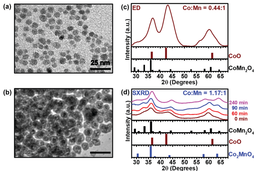
Fig. 1 Phase determination of \text{Co}_x\text{Mn}_{3-x}\text{O}_4\cdot(\text{CoO})_y NPs after oxidation for 90 min. (a) TEM image of oxidized spherical NPs for the Co : Mn molar ratio of 0.44 : 1. (b) TEM image of a second type of core-shell NPs present in the same sample shown in (a). (c) Integrated selected area electron diffraction (ED) pattern for image shown in (b). (d) Time series synchrotron X-ray diffraction (SXRD) patterns for the Co : Mn molar ratio of 1.17 : 1 NPs oxidized in air at 200 °C. SXRD pattern along with reference standards confirm the presence of CoO phase with contribution from spinel as well. The bar patterns in (c) and (d) show the reference XRD patterns for CoO (JCPDS: 00-048-1719), \text{CoMn}_2\text{O}_4 (JCPDS: 01-077-0471), and \text{Co}_2\text{MnO}_4 (JCPDS: 01-084-0482). Note: 2\theta scale for integrated ED is shifted to match Cu K_\alpha .
