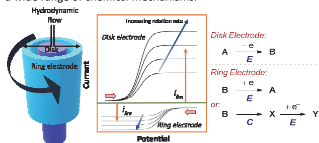
Figure 17. Schematic for an RRDE, demonstrating the typical current response at the disk electrode for a hypothetical oxidation reaction, followed by subsequent reduction at the ring. Each set of curves is separately measured by holding the potential at one electrode constant, whilst sweeping the potential at the other electrode across a given range. The figure displayed is thereby a composite of these two sets of experiments. Red arrows in figure demonstrate the direction of the scans, positive current represents oxidation.
