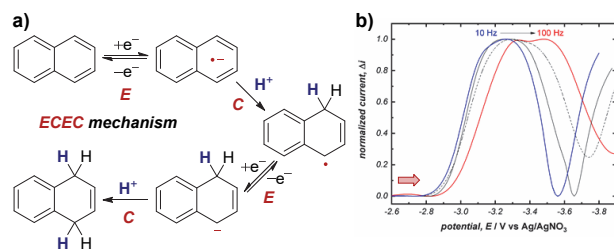
Figure 12. SWV study of the electrochemical Birch reduction of naphthalene provides evidence for two sequential electron-transfer steps, consistent with an ECEC mechanism, reported by the groups of Baran, Minter, Anderson and Neurock. Red arrow in figure demonstrates the direction of the scan, positive current represents reduction. Figure 12.b adapted with permission from reference 41. Copyright 2019 The American Association for the Advancement of Science.
