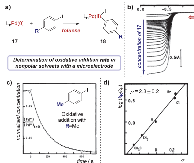
Figure 19. Measurement of oxidative addition rates of (\text{Ph}_3\text{P})_4\text{Pd}(0) , 17 , into para -substituted aryl iodides in toluene, reported by Amatore and Pflüger. b) Voltammograms measuring the oxidation of \text{Pd}(0) with varying concentrations of 17 at a gold-disk microelectrode. c) Calculation of the rate constant of oxidative addition for p -iodotoluene by plotting the concentration of 17 against time. d) Hammett plot of rate constants with different aryl iodides. Red arrow in figure 19.b demonstrates the direction of the scan, positive current represents reduction. Figure 19.b–d adapted with permission from reference 67. Copyright 1990 American Chemical Society.
