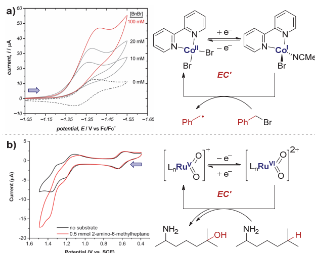
Figure 7. a) Evidence of electrocatalysis ( EC' mechanism) by a ligated Co(II) species through oxidative addition of benzyl bromide, reported by the groups of Minter and Sigman. Blue arrow in figure demonstrates the direction of the scan, positive current represents reduction. Adapted with permission from reference 20. Copyright 2019 American Chemical Society. b) Determination of catalytic Ru oxidation states from the increase in current due to catalysis, reported by the groups of Du Bois, Waymouth, Sigman and Zare. Blue arrow in figure demonstrates the direction of the scan, positive current represents reduction. Adapted with permission from reference 21. Copyright 2019 American Chemical Society.
