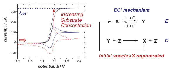
Figure 6. Representative CV responses for a catalytic ( EC' ) mechanism, demonstrating the change between peak-shaped response and plateau response as the substrate concentration increases. Simulations run with 0 equivalents (dashed red line), 10 equivalents (solid blue line) and 100 equivalents (solid black line) of substrate respectively. Arrow in figure demonstrates the direction of the scan, positive current represents oxidation.
