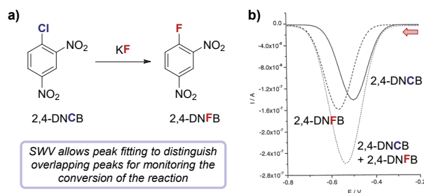
Figure 13. The conversion of the fluorination of 2,4-dinitrochlorobenzene (2,4-DNCB) can be monitored during the reaction by peak fitting reduction peaks using SWV, reported by Compton and co-workers. The signal for 2,4-DNFB (dashes) can be obtained by subtracting the signal of 2,4-DNCB (solid) from the combined SWV signal (dots). Red arrow in figure demonstrates the direction of the scan, positive current represents oxidation. Figure 13.b adapted with permission from reference 42. Copyright 2002 John Wiley and Sons.
