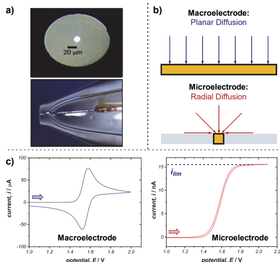
Figure 18. a) Optical microscope images of the top and side of an exemplar microelectrode. b) The difference in transport to a macro- and microelectrode results in differing voltammetric responses, shown for a representative reversible oxidation in c). Arrows in figure 18.c demonstrate the direction of the scan, positive current represents oxidation. Figure 18.a adapted with permission from reference 65c. Copyright 2006 Institute of Physics Publishing
