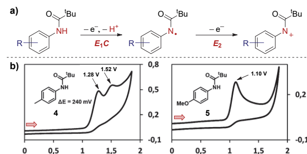
Figure 3. CV responses displaying the dependence of the separation in potential of the two electron oxidation processes on the structure of the anilide, reported by Waldvogel and co-workers. Red arrows in figures demonstrate the direction of the scan, positive current represents oxidation. Figure 3.b adapted with permission from reference 13. Copyright 2017 American Chemical Society.
