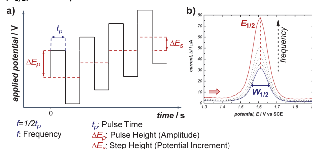
Figure 11. a) Staircase-shaped waveform of a SWV experiment. b) "Bell-shaped" curve that results from the signal of a chemically reversible redox couple of an electroactive species in a SWV experiment (cf., representative CV response in Figure 1.b). Red arrow in figure 11.b) demonstrates the direction of the scan, positive current represents oxidation.
