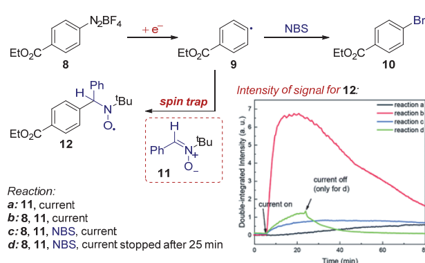
Figure 15. EPR spectroelectrochemistry provides evidence for the formation of radical 9 following electrochemical reduction, and the subsequent reaction with N -bromosuccinimide (NBS), reported by Mo and co-workers. The formation of radical 9 is measured by the EPR signal of the long-lived radical 12 afforded by spin-trapping. Adapted with permission from reference 50. Copyright 2018 The Royal Society of Chemistry.
