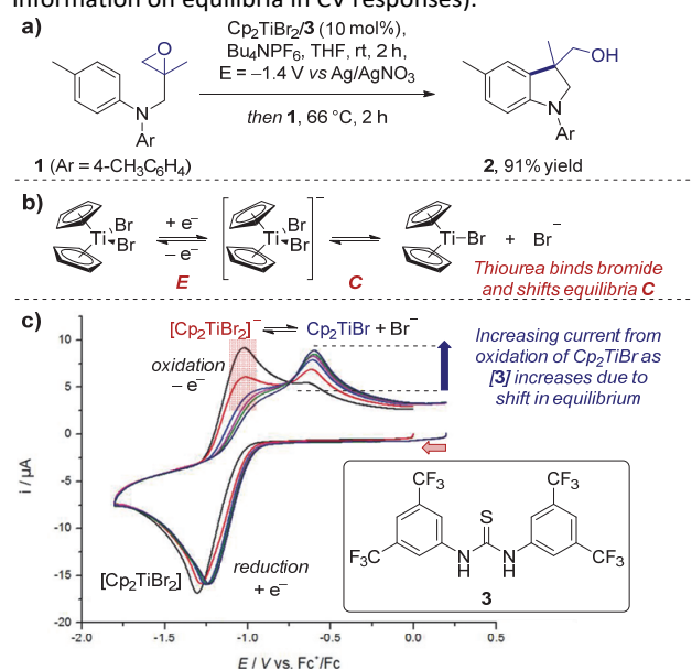
Figure 2. An example of CV used to monitor the speciation of the active titanocene catalyst ( \text{Cp}_2\text{TiBr} ), depending on the equivalents of thiourea 3 added, utilised in a radical epoxide arylation by Gansäuer and co-workers. Red arrow in figure demonstrates the direction of the scan, positive current represents oxidation. Figure 2.c adapted with permission from reference 12a. Copyright 2018 John Wiley and Sons.
