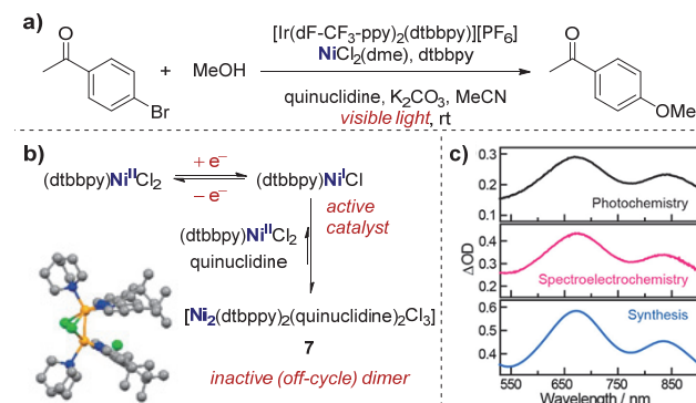
Figure 14. Evidence for the formation of a mixed-valent Ni(I/II) dimer ( 7 ) in the photochemical etherification of arylhalides, reported by Nocera and co-workers. 7 was synthesised independently, and the corresponding UV-Vis profile found to match measurements made of the reaction mixture in both photochemical and spectroelectrochemical settings (Figure 14.c). Figure 14.b and 14.c adapted with permission from reference 48. Copyright 2019 American Chemical Society.
