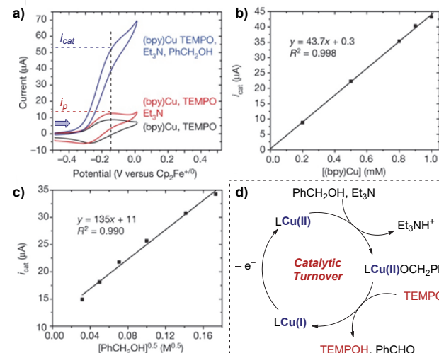
Figure 9. Kinetic studies of a cooperative electrocatalytic alcohol oxidation by measuring the catalytic current on a CV response as a function of substrate/catalyst concentration, reported by Badalyan and Stahl. Blue arrow in figure demonstrates the direction of the scan, positive current represents oxidation. Figure 9.a–c adapted with permission from reference 28. Copyright 2016 Springer Nature.
