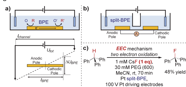
Figure 24. a) Schematic of a bipolar electrochemical set-up, demonstrating the formation of anodic and cathodic poles on a bipolar electrode (BPE). b) Schematic of a split-bipolar electrode in a U-type cell. c) Fluorination of triphenylmethane can occur at low concentrations of electrolyte solution utilising a BPE set-up, reported by Inagi and co-workers [Reference 83; poly(ethyleneglycol) (PEG) additive required to solubilise CsF in acetonitrile].
