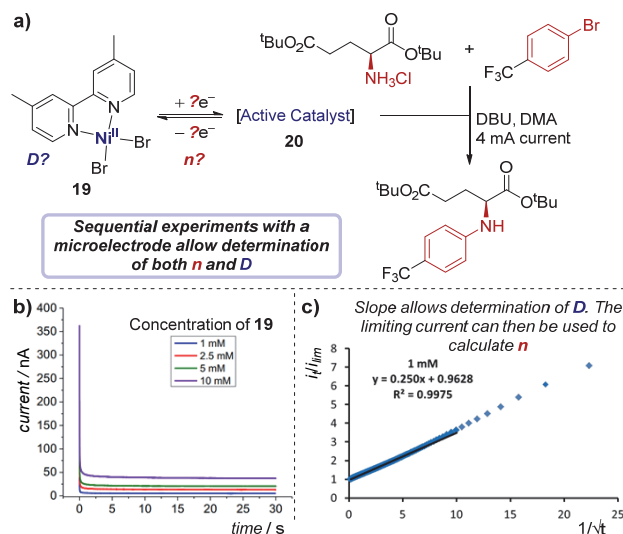
Figure 20. Determination of both the diffusion coefficient and number of electrons transferred in the reduction of 19 , by the groups of Baran, Minter, Neurock and White. The current response upon application of a potential step is measured, b ), and the slope of the plot in c ) allows determination of the diffusion coefficient. Positive current represents reduction. Figure 20.b–c adapted with permission from reference 39c. Copyright 2019 American Chemical Society.
