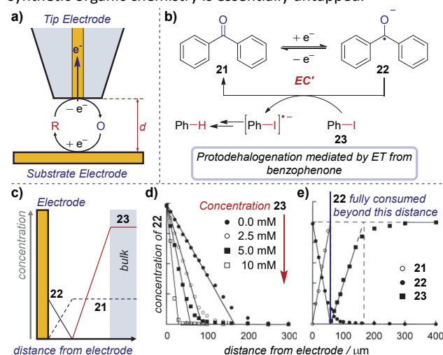
Figure 22. a) Schematic of an SECM set-up, where the distance ( d ) between the substrate and tip electrodes can be changed to measure concentrations in solution. The concentration profile of species in the mediated reduction of iodobenzene, b), measured by Amatore et al. using SECM. c) Schematic of concentration profiles. d) Concentration profile of 22 with varying equivalents of 23 , measured by changing the distance ( d ) between the two electrodes. e) Comparative concentration profile of various species in solution. Figure 22.c–e adapted with permission from reference 75. Copyright 2001 John Wiley and Sons.
