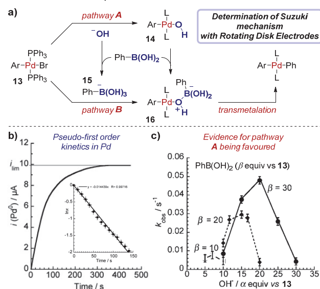
Figure 16. RDE experiments provide evidence for a palladium-hydroxyl species as a catalytic intermediate in the Suzuki cross-coupling reaction, reported by Amatore et al. For inset in b ), x is the fractional conversion to Pd(0). Figure 16.a adapted with permission from reference 58. Copyright 2013 John Wiley and Sons. Figure 16.b and 16.c adapted with permission from reference 57. Copyright 2011 John Wiley and Sons.
