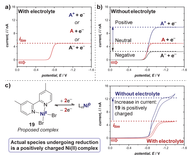
Figure 21. Representative microelectrode voltammograms of the reduction of species A with unknown charge at a microelectrode, a ) in the presence of supporting electrolyte, and b ) in the absence of supporting electrolyte, wherein the limiting current of the voltammogram changes depending on the charge of the species undergoing reduction. c ) Measurement of the limiting current of the two-electron reduction of proposed complex 19 (cf., Figure 20) with and without electrolyte demonstrates that the complex bears a positive charge, by White and co-workers [reference 72]. Red arrows in figure demonstrate the direction of the scan, positive current represents reduction.
