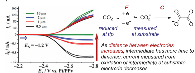
Figure 23. SECM study of the reduction of carbon dioxide allows detection of the short-lived radical anion intermediate, reported by Bard and co-workers. Blue arrow in figure demonstrates the direction of the scan, positive current represents reduction. Adapted with permission from reference 78a. Copyright 2017 American Chemical Society.
