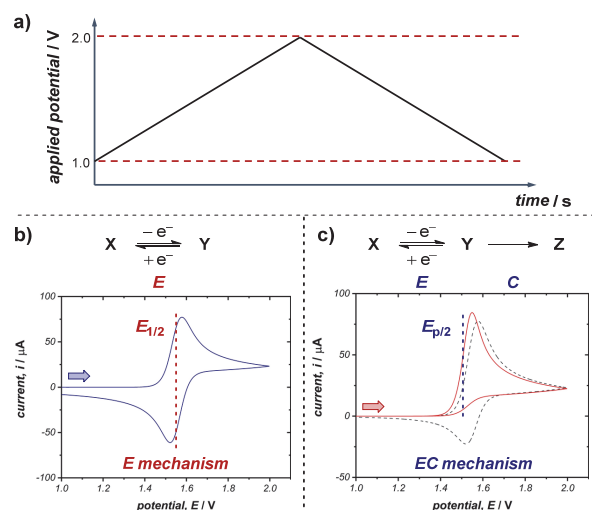
Figure 1. a) Example of a triangular potential waveform applied in the generation of a cyclic voltammogram. Representative CV responses for b) a chemically reversible electron transfer (E mechanism), and c) a chemically irreversible electron transfer in which the redox event is followed by a chemical reaction (EC mechanism). Two lines in c) represent different rates of the following chemical reaction, where the dashed grey line has a rate constant of 0.1 \text{ s}^{-1} and the solid red line a rate constant of 10 \text{ s}^{-1} (with E_{p/2} labelled for the latter). Arrows in figures demonstrate the direction of the scan, positive current represents oxidation.
