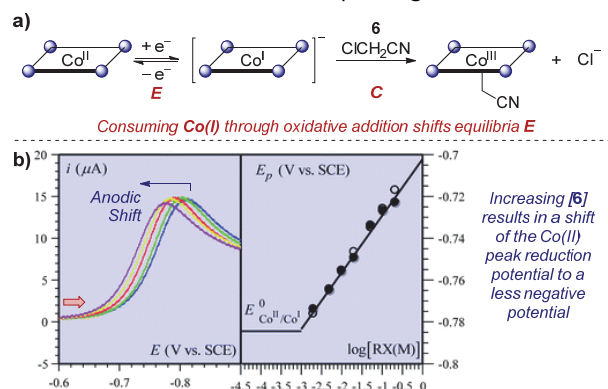
Figure 10. Kinetic studies on the rate of oxidative addition of chloroacetonitrile 6 to cobalt(I) tetraphenylporphyrin (ligand depicted by the four nitrogen binding sites as circles), reported by Costentin et al. The shift in the peak reduction potential by the concentration of chloroacetonitrile (RX in b ) allowed determination of the rate constant. Red arrow in figure demonstrates the direction of the scan, positive current represents reduction. Figure 10.b adapted with permission from reference 35. Copyright 2013 The Royal Society of Chemistry.
