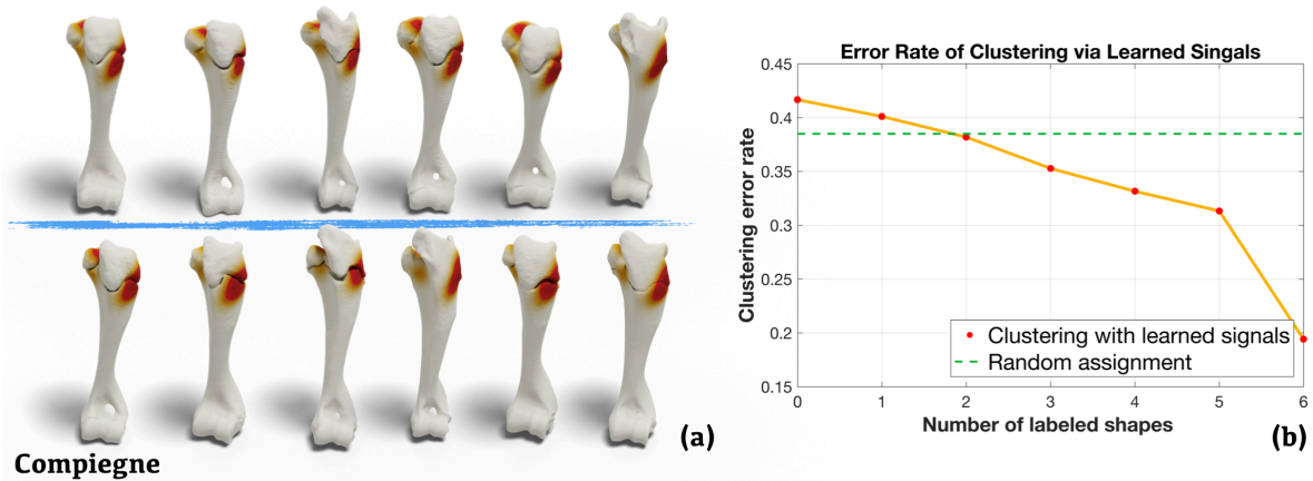
Figure 10: (a) comparing two sets of bones corresponding to different populations of wild boars using computed functional maps; (b) error rates of clustering via the distinctive signals computed with different number of labeled data in a semi-supervised learning setting. See text for details.
