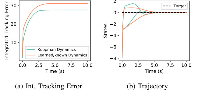
Fig. 1: Control performance of a forced van der pol oscillator with an LQR control using the learned Koopman operator, the linearization of the known system dynamics, and the linearization of a learned state-space model using the same data and basis functions as the Koopman operator. The control performance using the Koopman operator dynamics is shown to outperform the LQR control with known dynamics. The learned dynamics model performs equally to the known dynamics model and is overlaid on top of the known dynamics results.
