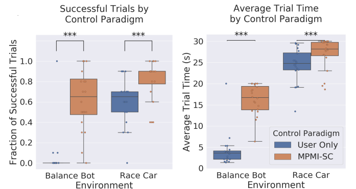
Fig. 3: Average success rate (left) and average time to failure (right), broken down by environment and control paradigm. The maximum interaction time was 20s in the balance bot and 30s in the race car. Both metrics improve significantly (***) : p < 0.005 ) under shared control.
