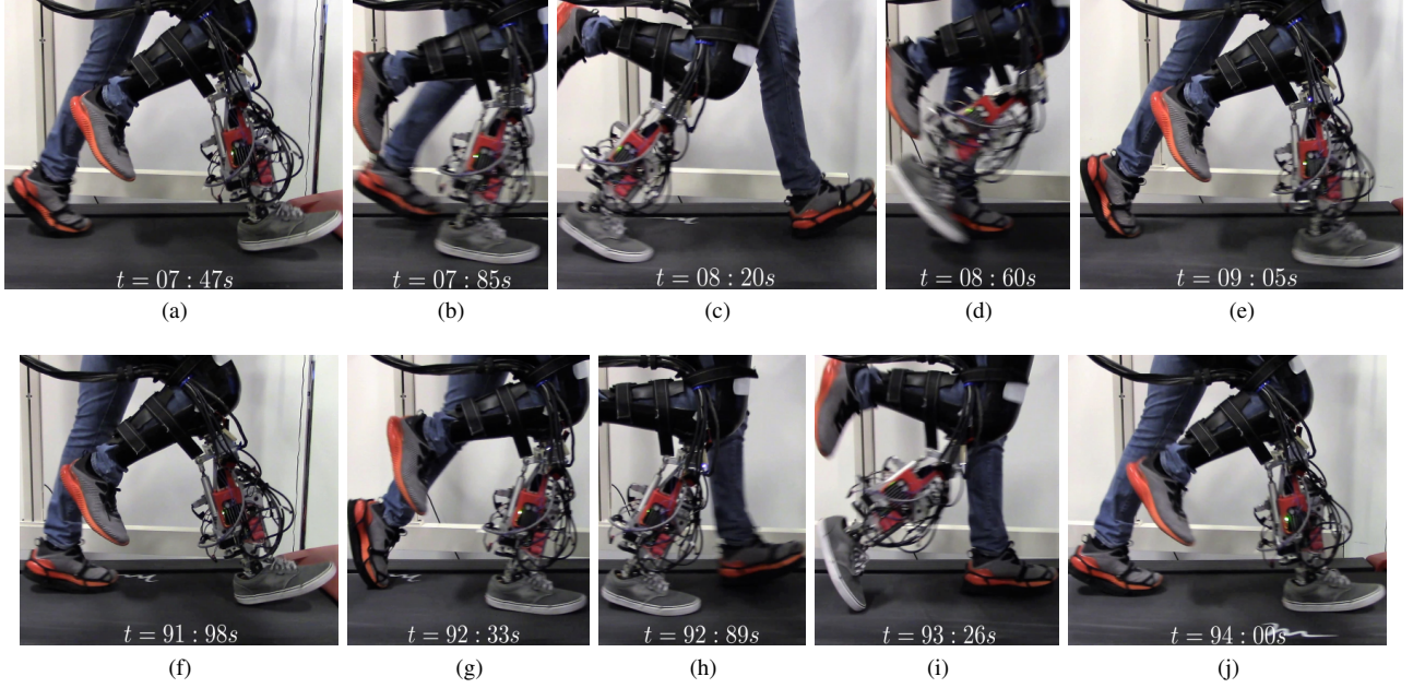
Fig. 10: Snapshots of walking experiments. Figs. 10a-10e show the photos of fast walking experiments at 1.34 \text{ m/s} , and Figs. 10f-10j show the photos of slow walking experiments at 0.89 \text{ m/s} for one gait cycle. A supplemental video of the experiment is available for download.
