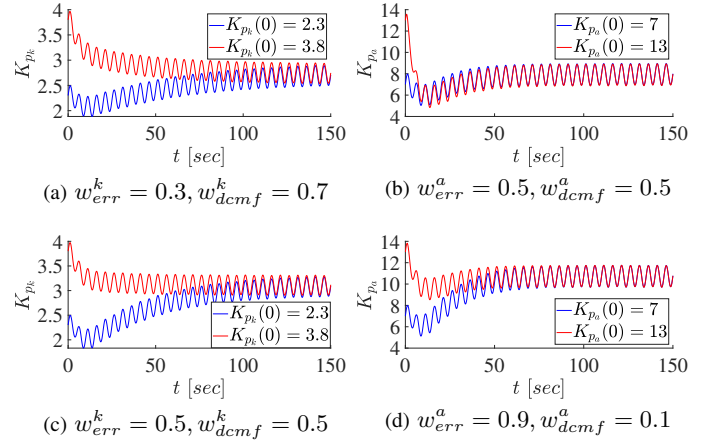
Fig. 7: Simultaneous ESC adaptation of K_{p_k} and K_{p_a} , starting from different initial conditions and different convex combinations of objective functions. The convergence to the same optimum K_{p_i}^* , starting from different initial K_{p_i} experimentally verified the convexity of the cost function, developed in Section III-B. Also, it can be seen that when J_{err}^i was weighed higher, K_{p_i} converged to a higher value.
