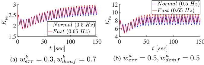
Fig. 9: Benchmark experimental results showing simultaneous ESC adaptation of K_{pk} and K_{pa} , for different speeds. It can be seen that K_{pi} converges to a higher value for faster trajectories.
