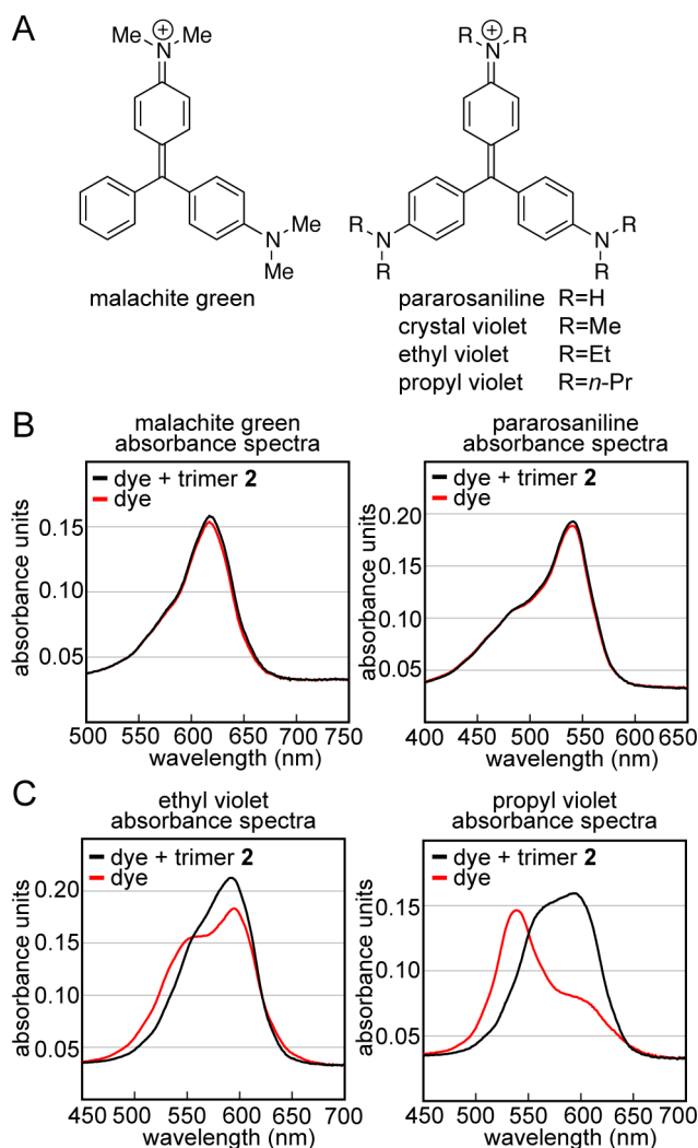
Figure 5: Interaction of other triphenylmethane dyes with trimer 2 . (A) Chemical structures of crystal violet and related triphenylmethane dyes. (B) Absorbance spectra of 25 \mu\text{M} malachite green and 25 \mu\text{M} pararosanaline in the presence (black) or absence (red) of equimolar trimer 2 . (C) Absorbance spectra of 25 \mu\text{M} ethyl violet and 20 \mu\text{M} propyl violet in the presence (black) or absence (red) of equimolar trimer 2 . Experiments were performed in buffer comprising 50 mM sodium acetate and 50 mM acetic acid (pH 4.6).
