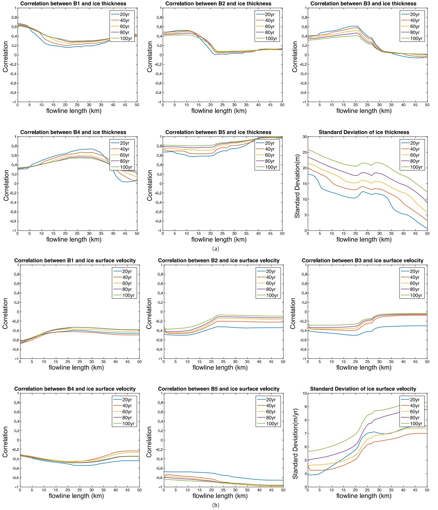
Fig. 3. (a) Results of Experiment 2, independently varying friction B1, ..., B5. Shown are the correlation between B for each section and ice thickness, as indicated, together with the standard deviation of thickness (lower right). (b) As in Fig. 3a, but showing the correlation to surface velocity u , and the standard deviation of the surface velocity.
