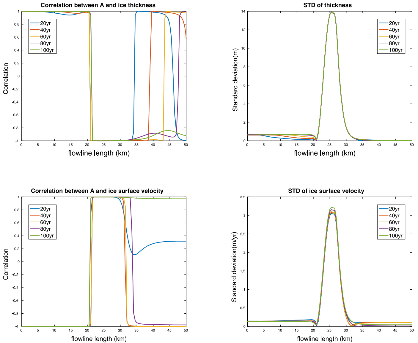
Fig. 2. Results of Experiment 1a, varying terrain height A. Shown are the correlation between A and ice thickness (upper left) and surface velocity u (lower left), and standard deviations of thickness (upper right) and velocity (lower right).
