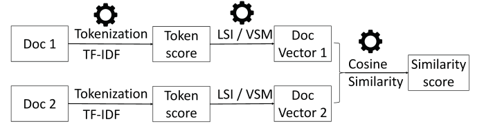
Figure 5: Calculating similarity for description / patch content
