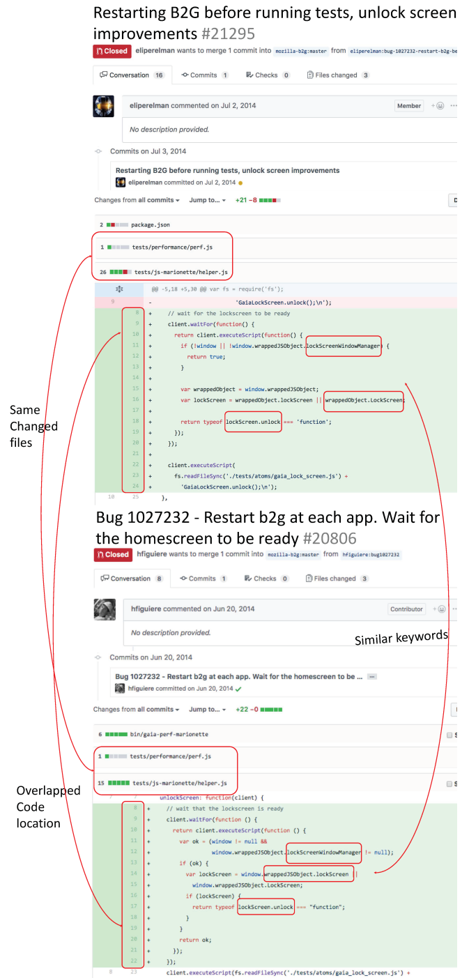
Figure 4: Duplicate PRs with similar code change information duplicate of. We then went through each pair of duplicate pull requests and inspected the text and code change information to extract clues indicating the potential duplication. The first two authors iteratively refined the clues until analyzing more duplicate pairs yielded no further clues.
