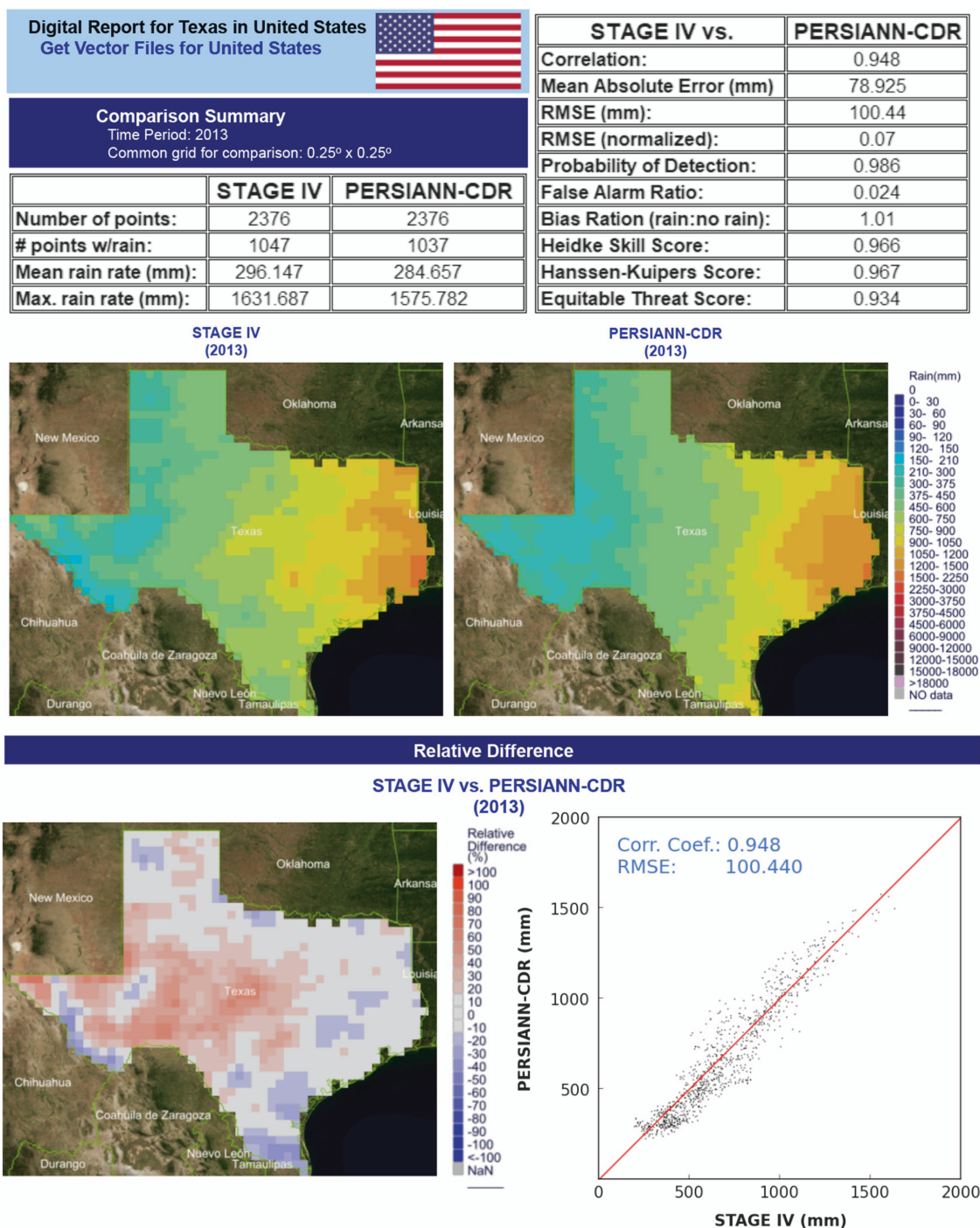
Figure 2. An example of the auto-generated reports created by the Comparison tool.
