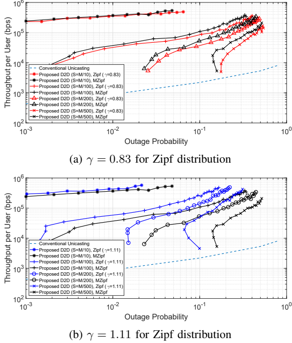
Fig. 5: Throughput outage tradeoff comparisons between different models for Metro region 2 of July in networks assuming mixed office scenario for propagation channel; varying local storage size.
