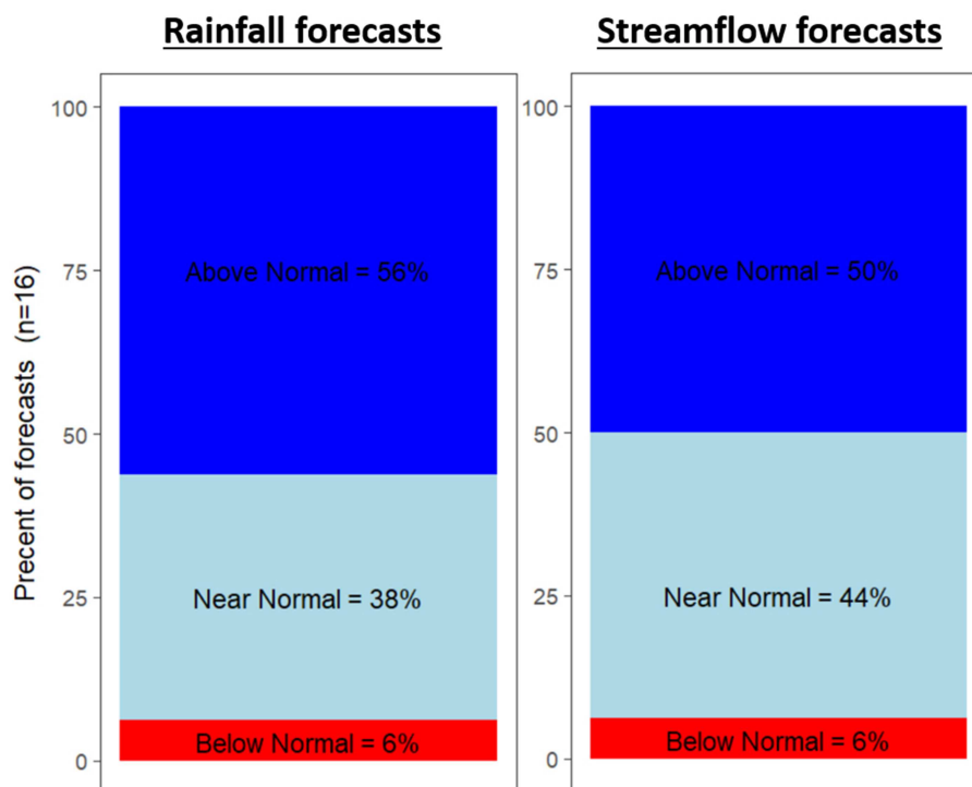
FIGURE 4 | Percentage of forecasts in this study predicting below normal, near normal, and above normal June–September rainfall ( Left ) and June–December streamflow at the GERD site ( Right ) for 2018, including eight NMME models (ensemble mean for each model) and eight statistical models. NMME forecasts are adjusted for mean biases. No variance adjustment was applied to any of the model forecasts.
