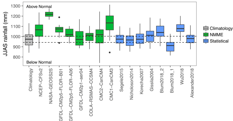
FIGURE 5 | Boxplots (representing the 25th–75th percentiles and with whiskers extending to 1.5 times this interquartile range) of rainfall forecasts by model, illustrating NMME ensemble spread and statistical models prediction with 100 randomly-selected residuals. Dashed lines show below/above normal conditions. Statistical boxes represent range of 2018 forecast plus 100 resampled errors (from 1982 to 2017 leave-one-out predictions).
