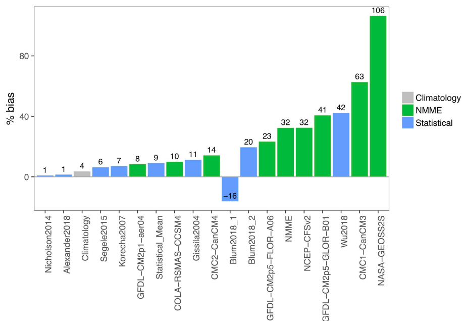
FIGURE 7 | Percent bias of each 2018 GERD inflow streamflow forecast relative to 2018 estimated streamflow of 41,180 million m 3 /month (based on observed CHIRPS rainfall). Numbers at the top of the bars give the % bias associated with each forecast. The bar labeled NMME refers to the mean of all NMME predictions and the bar labeled Statistical_Mean refers to the mean of all of the statistical models.
