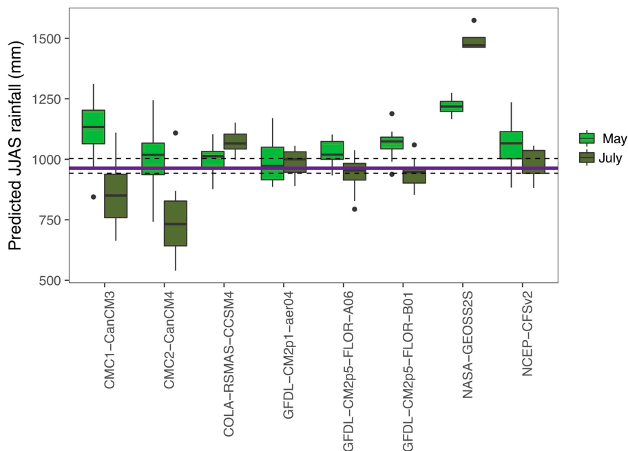
FIGURE 8 | Comparison of GERD basin June–September 2018 rainfall forecasts forecasted in May 2018 (also plotted in Figure 5 ) and in July 2018. The horizontal purple line indicates CHIRPS estimate of total rainfall 963 mm.
