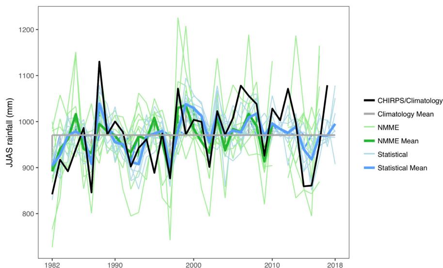
FIGURE 3 | 1982–2017 hindcasts for June–September Upper Blue Nile GERD basin rainfall. Light blue lines are statistical models, with the darker blue line showing the ensemble average of statistical models applied in this project. Green lines are NMME forecasts initialized in May of each year—each light green line is the ensemble average of a single model and the dark green line is the full NMME ensemble average for all models that had complete data records (other than 2011 and 2017 which were unavailable for all models). The black line shows the CHIRPS total June–September rainfall in each year and the gray horizontal line shows the average across the record.
