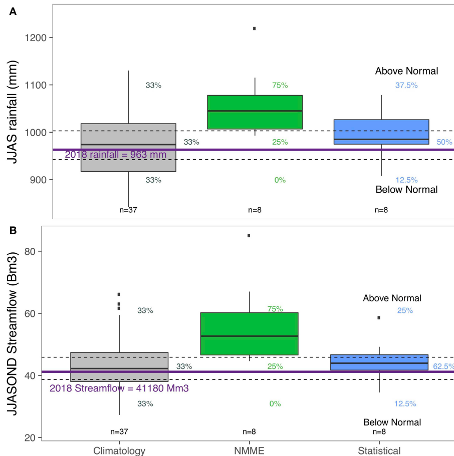
FIGURE 6 | (A) Boxplots of June–September historical rainfall, 1982–2017, according to CHIRPS rainfall estimates (gray), and of the 2018 forecasts for dynamically-based models participating in the North American Multimodel Ensemble (NMME; green) and for statistically-based models applied in this study (blue). Dashed lines show the upper and lower terciles of historical rainfall totals and percentages indicate the percent of each streamflow within each tercile, corresponding to the closest box and with matching color. (B) As in (A) , but for the June–December 2018 calibrated and forecast Upper Blue Nile streamflow at the GERD site.
