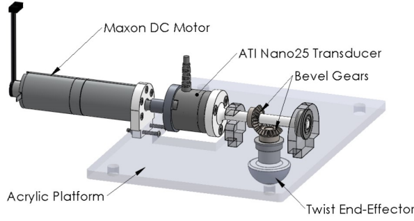
Fig. 4. Isometric view of twist module. While the direction of action differs from that of the stretch and squeeze modules, the loads involved can be measured by the same sensor configurations.
