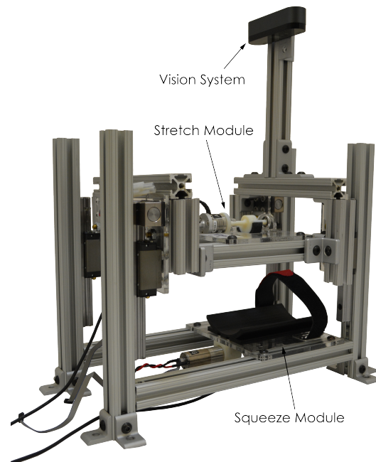
Fig. 1. A modular haptic testbed has been developed to allow for evaluation of single and multi-sensory tactile cues. The testbed integrates various sensing modalities to characterize the device interactions with the human user, and to facilitate psychophysical evaluations.
