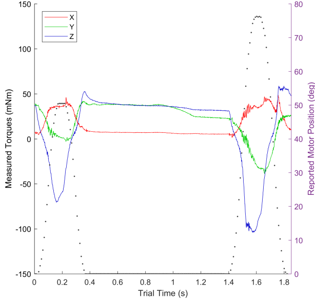
Fig. 5. Stretch module motor position in degrees overlayed onto x-, y- and z- axis torque outputs when stretch module is driven to 52^\circ , back to 0^\circ , waiting for 1 second then driving to 78^\circ before finally returning to 0^\circ . The force and torque data were reported from the sensors at 1000 Hz and the position data were reported from the motor controller at 100 Hz. Note that the PID controller operates at 2500 Hz; the 100 Hz reporting is due to hardware bandwidth limitations.
