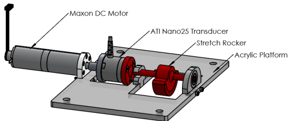
Fig. 2. Isometric view of stretch cue module. The stretch mechanism is driven by a DC motor with a force-torque sensor placed in series, allowing for accurate measurement of the loads exerted on the subject's forearm.
