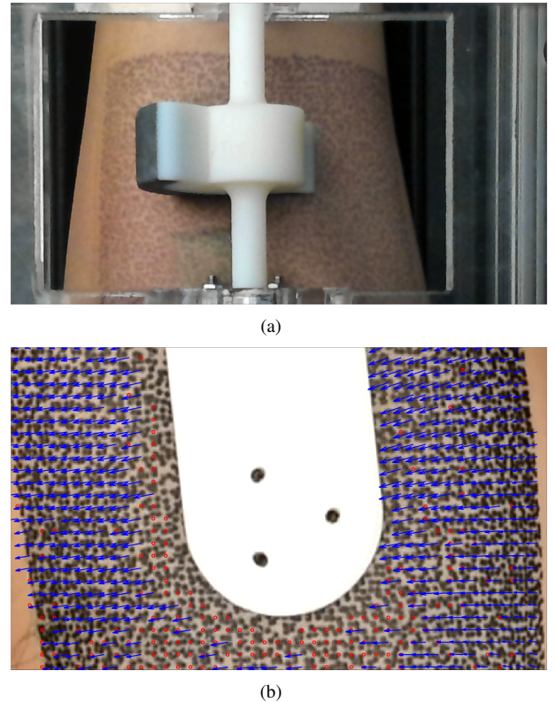
Fig. 6. (a) Still frame from experimental video data focused on the region of interaction of the stretch device. The ink pattern seen is a speckle pattern stamped onto the skin using skin-safe temporary tattoo ink and a custom-made stamp. This pattern can be used with digital image correlation algorithms to determine the effects of stretch intensity on skin deformation and rocker slippage - a secondary goal of the experiment performed. (b) Example tracking of speckle pattern on skin using Digital Image Correlation Engine (DICE).
