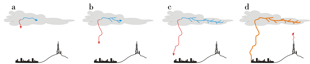
Figure 8. (a) Bidirectional intracloud leader development begins with positive (red) and negative (blue) leaders expanding from an initiation point (b,c). The positive leader approaches the ground prior to initiating a return stroke with the negative end of the leader passing near the tower (d). The return stroke traverses the leader network and initiates an upward positive leader from the tower (red rising leader).
