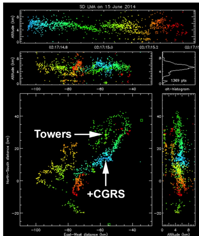
Figure 2. LMA source data plot of an upward flash on 15 June 2014 at 02:17:14 UT. Green + signs are tower locations.
