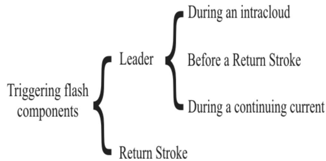
Figure 5. Triggering flash components that cause the upward leader initiation.
