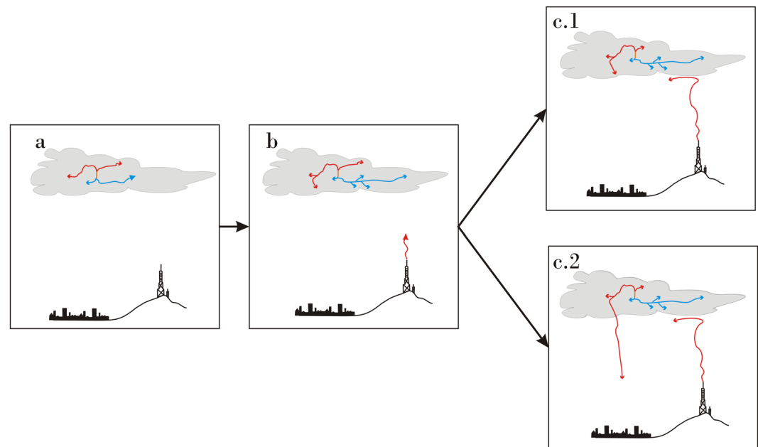
Figure 6. (a) Bidirectional intracloud leader development begins with positive (red) and negative (blue) leaders expanding from an initiation point. (b) The approach of negative leader initiates and upward positive leader (red) during an intracloud flash (c.1) or prior to a return stroke of a CG flash (c.2).
