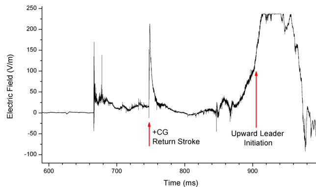
Figure 3. INPE fast antenna data plot from 15 June 2014 at 02:17:14 UT.
