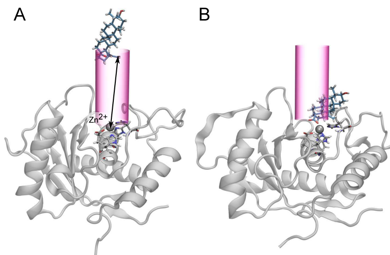
Figure 4. Schematic representation of the cylindrical restraint potential used in the free-energy calculations, similar to the funnel metadynamics protocol [30]. The carboxylate of the triterpenic acids (or C-17 hydroxyl of betulin) was subject to a restraining force when its distance from the cylindrical axis (centered on the \text{Zn}^{2+} ion) exceeded 4.5 Å. This distance was sufficiently large that the restraining force was never active when the carboxylate– \text{Zn}^{2+} distance was near the free energy minima ( r < 3.5 Å); therefore, it should not have influenced sampling of the bound state. The only exception was betulin, which possesses no carboxylate and exhibited marginal affinity for the active site. (A) An unbound state of betulinic acid and BaP1. The arrow represents the transition coordinate, r , defined as the distance between the carboxylate group and the \text{Zn}^{2+} ion. (B) A bound state of betulinic acid, with r = 2.8 Å.
