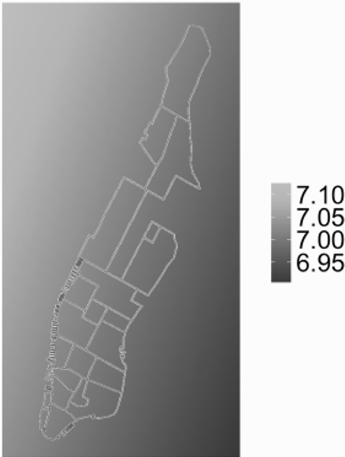
Fig 19. Estimated function of spatial trend of Manhattan.
