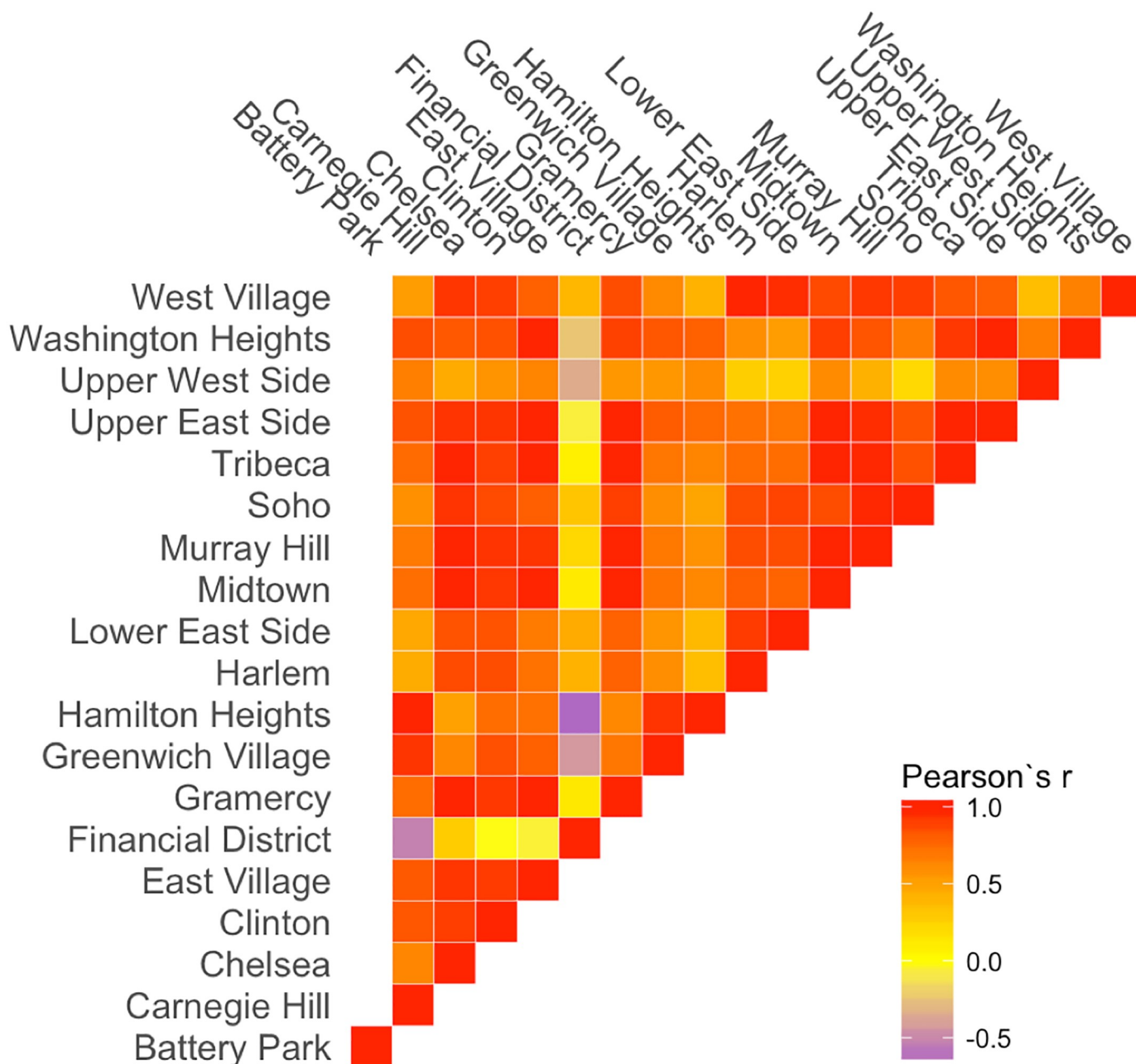
Fig 4. Pairwise Pearson correlation of neighborhoods' coffee shop densities.
