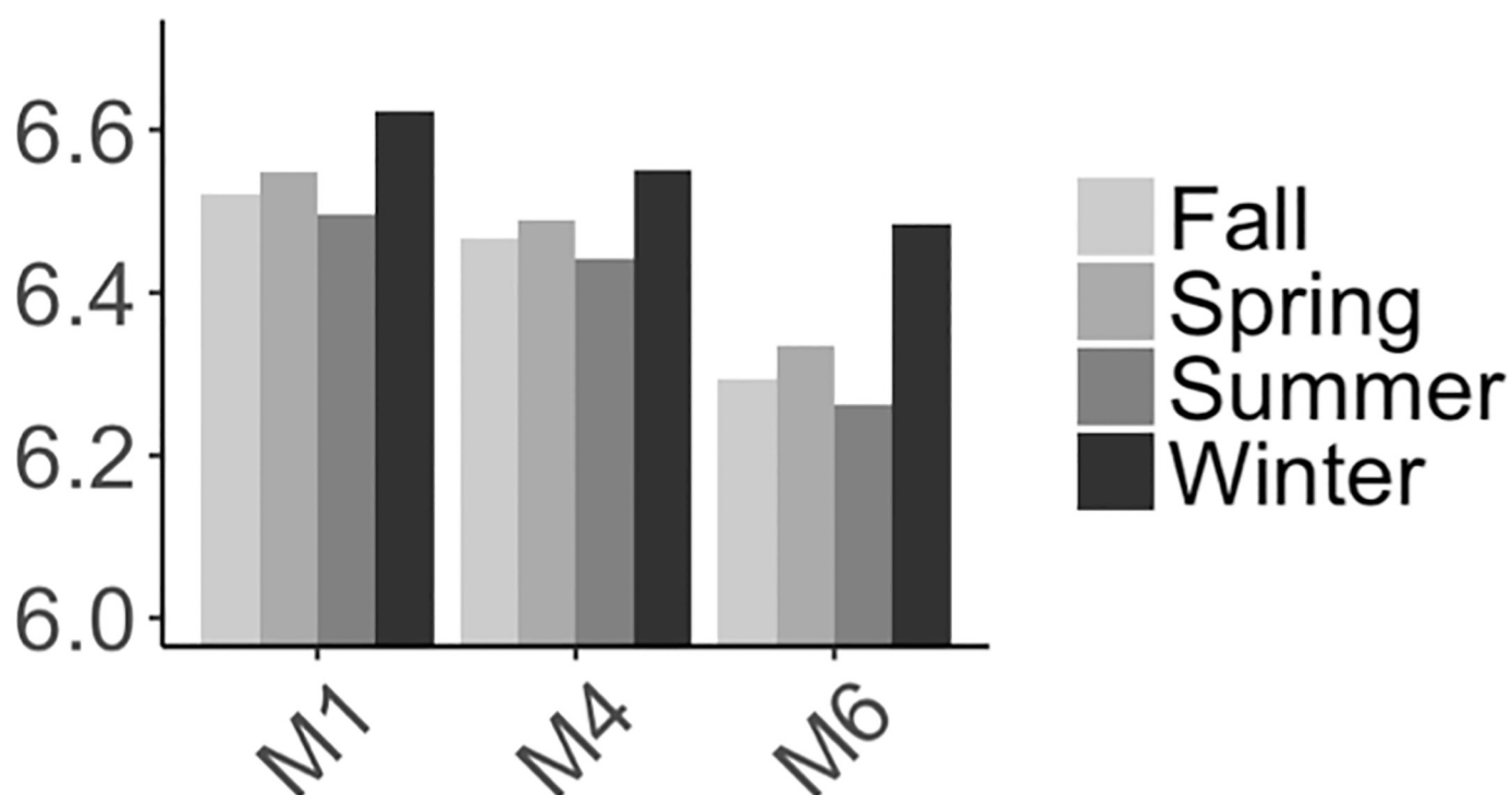
Fig 18. Estimated coefficients of seasonal trend of Manhattan.
