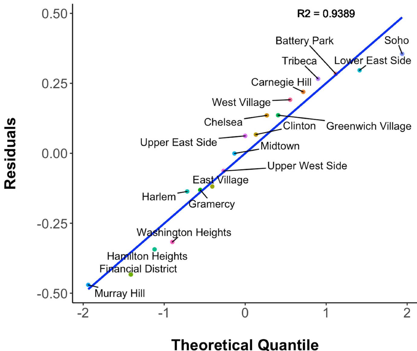
Fig 16. Q-Q plot of residuals of scaling relationship model.
