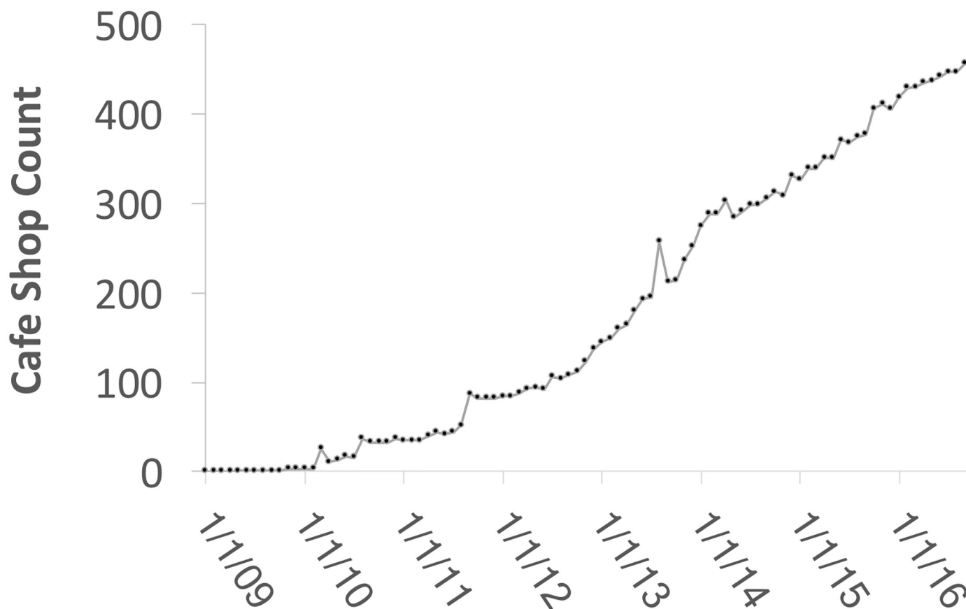
Fig 2. Coffee shop count in Manhattan from OSM—Monthly 1/1/2009–11/31/2016.
