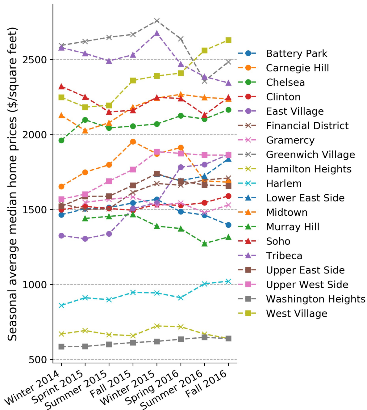
Fig 7. Unit home price (UHP) ($/ft 2 ) changes—Seasonal average 12/2014–11/2016.
