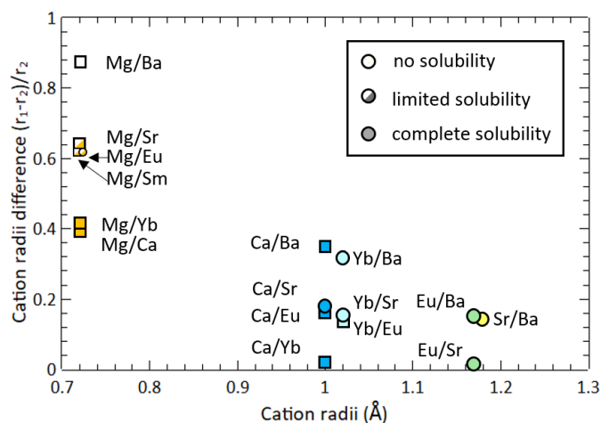
Figure 4. The cation radii difference of \text{AM}_2\text{X}_2 calculated from (r_1 - r_2)/r_2 for all possible combinations of cations where r_1 > r_2 . In each combination, the smaller species is listed first. Square symbols represent experimental observations, while circles represent predictions. The limited solubility in Sr/Mg (present study) and Sm/Mg (Reference [36]) alloys provide an approximate upper limit for cation radii mismatch. The complete solubility of Ca/Eu [19,20,24], Ca/Yb [20–22,26], and Yb/Eu [20,23] Mg/Yb [25] have been confirmed by prior studies.
