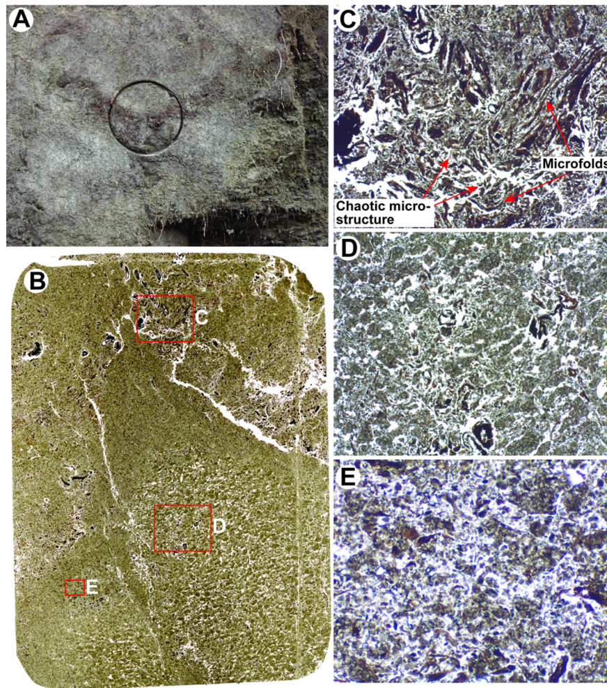
Figure 20 Microstructures in palaeosol complex 1 within yedoma silt of unit 4, thin section 4, 6.5 m arl. (A) Upper of three root-rich layers, showing involuted organic-rich lens (palaeosol) in the centre and numerous in-situ roots, the larger ones (upper right) woody. Imprinted circle (9 cm diameter) marks the location of the sediment sample from which thin section 4 (B) was obtained. (B) Organic-rich silt within involuted lens, showing locally high concentrations of organic material (dark brown) and textural heterogeneity attributed to cryoturbation. (C) Root-rich silt containing (1) microfolds that are picked out by elongate roots and (2) a chaotic microstructure of fragmented and irregularly oriented organic material and aggregates. (D) Aggregates of about 0.3–2 mm maximum dimension surrounded by an irregular pore network (white) that represents a former microcryostructure transitional between irregular reticulate and pore. (E) Aggregates of about 0.1–1 mm maximum dimension and interspersed particles of mineral and humic material. The former microcryostructure is pore, indicated by the irregular pore network. Scanned thin section in (B) is 47 mm wide x 64 mm high, in correct vertical orientation. Photomicrograph frame widths in (C), (D) and (E) are 8.3, 8.3 and 2.6 mm, respectively. arl = Above river level. This figure is available in colour online at wileyonlinelibrary.com/journal/ppp
