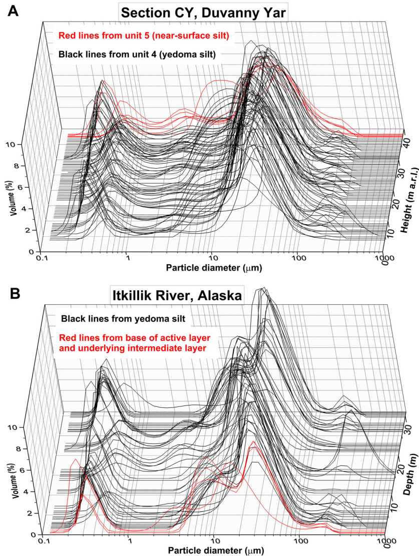
Figure 15 Particle-size distributions (PSDs) of yedoma silt of unit 4 plotted (A) against height above river level (arl) for Duvanny Yar and (B) against depth below the ground surface for the Itkillik River. In (A) PSDs are for samples 9–14, 16–54 and 56–82 from section CY. Red lines are from samples 71–76 in unit 5 (near-surface silt); black lines are from unit 4 (yedoma silt). In (B) PSDs are for samples 1–3, 5–9 and 11–54. The red line at the shallowest depth indicates a sample from the base of the active layer, and the others indicate samples from the underlying intermediate layer. The black lines are for samples from underlying yedoma silt of units 3 and 4 (see Table 6). This figure is available in colour online at wileyonlinelibrary.com/journal/ppp
