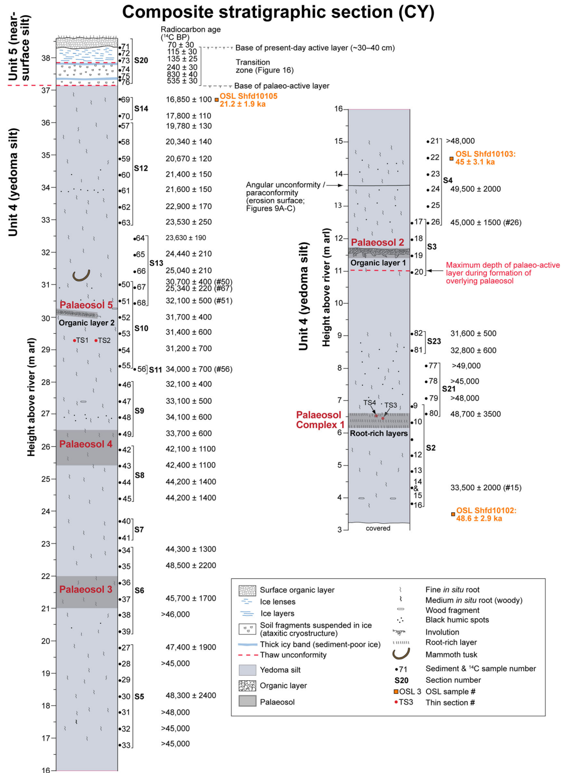
Figure 5 Composite stratigraphic section (section CY) examined in 2009 at Duvanny Yar, showing relative vertical position of the 16 individual sections through units 4 (yedoma silt) and 5 (near-surface silt). Sample locations indicated. S2 to S23 indicate individual section numbers within the composite section CY. arl = Above river level. This figure is available in colour online at wileyonlinelibrary.com/journal/ppp
