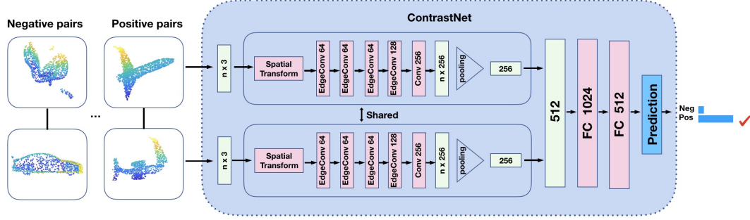
Figure 3. The architecture of ContrastNet for part contrast learning. The positive pair is generated by randomly sampling two segments from the same point cloud sample, while the negative pair is generated by randomly sampling two segments from two different samples. A dynamic graph convolution neural network (GNN) is used as the backbone network. The features of two segments are concatenated and fed to fully connected layers to make the prediction of positive or negative. The part contrast learning does not require any data annotations by humans.
