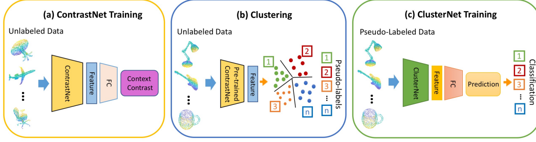
Figure 2. The proposed unsupervised feature learning includes three main steps: (a) ContrastNet for part contrast learning, by verifying whether two point cloud cuts belong to the same object; (b) Clustering samples of 3D objects and assign cluster IDs, using the features learned by ContrastNet; (c) ClusterNet for object clustering learning, by training the network with the 3D point cloud data while the labels are the cluster IDs assigned by the clustering step.
