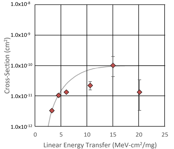
Fig. 7. Weibull curve for configuration memory cell upsets, per bit. Error bars that are smaller than the marker symbol may not be visible. The Weibull parameters are L_{th}=1.5 [MeV-cm 2 /mg], \sigma_{sat}=0.01 [ \mu\text{m}^2/\text{bit} ], W=8.0 [MeV-cm 2 /mg], S=2.2 .
