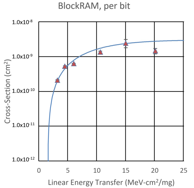
Fig. 11. Weibull curve for BlockRAM upsets, per bit. Error bars that are smaller than the marker symbol may not be visible. The Weibull parameters are L_{th}=1.5 [MeV-cm 2 /mg], \sigma_{sat}=0.3 [ \mu\text{m}^2/\text{bit} ], W=10.0 [MeV-cm 2 /mg], S=1.5 .
