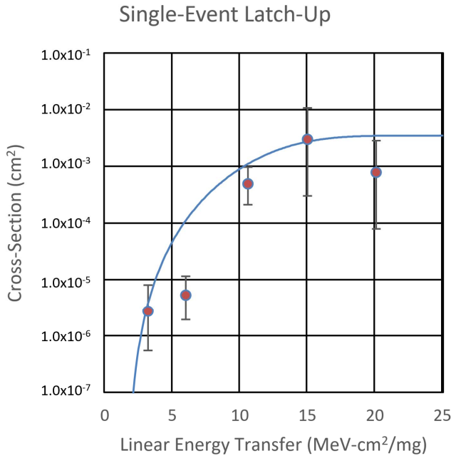
Fig. 13. Weibull curve for single-event latch-up events. The Weibull parameters are L_{th}=1.5 [MeV-cm²/mg], \sigma_{sat}=3.5 \times 10^5 [ \mu\text{m}^2/\text{bit} ], W=12.0 [MeV-cm²/mg], S=3.5 .
