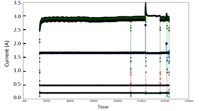
Fig. 14. Current plot of one test segment. Change in current was 600 mA on the top plot and 1 A on the upper-middle plot.
