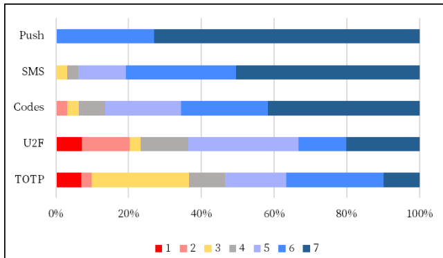
Figure 5: SEQ scores for five 2FA methods.
