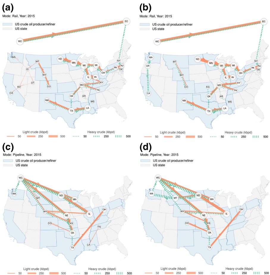
Fig. 9 A Rail flows in the base case, 2015 b 2015 rail flows in the scenario “US Midwest Pipeline Investments” in which new pipelines are built to convey oil from North Dakota both to the east and west. c Pipeline flows in the base case, 2015 (D) Pipeline flows of crude oil in 2015 under the scenario “US Midwest Pipeline Investments”
