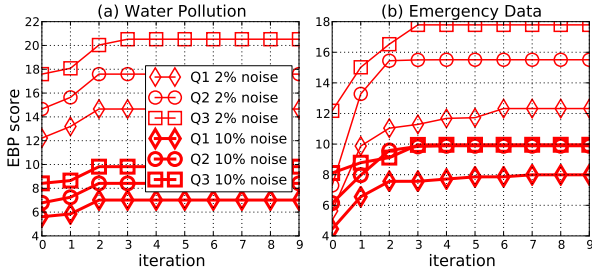
Figure 4: Efficiency Measure: Evolving curves of graph scan statistic scores (EBP) for our method (Query-map) in different iterations. These scores are evaluated on these two datasets with 2% and 10% noises and the query graphs.
