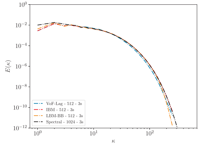
Fig. 6. Spectra for single-phase case for two given times. Top: t = 1.25 T_0^e (1 s); Bottom: t = 3.75 T_0^e (3 s).
