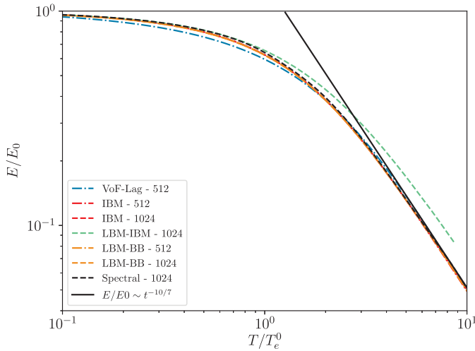
Fig. 5. Decaying fluid kinetic energy of single-phase flow. E_0 and T_0^e denote the values of kinetic energy and eddy turnover time at T = 0 , respectively.
