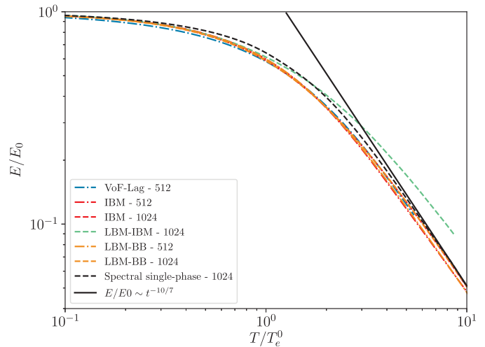
Fig. 8. Decaying fluid kinetic energy of two-phase flow. E_0 and T_e^0 denote the values of kinetic energy and eddy turnover time at T = 0 , respectively.
