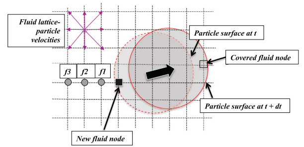
Fig. 3. Sketch to illustrate the key ideas for treating the fluid-solid interface in LBM-BB. The interpolated bounce-back scheme constructs an unknown distribution at a boundary node f_1 , at time t , in terms of known distributions at f_1 and other nearby fluid nodes (say f_2 and f_3 ) as needed. The refilling would create distribution functions at the new fluid node. The momentum exchange algorithm then sums up the net momentum exchange at the all boundary nodes with links cutting through the surface of a solid particle.
