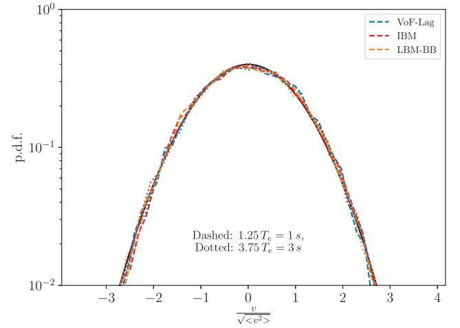
Fig. 10. P.D.F. of particle velocity averaged over 3 velocity components.
