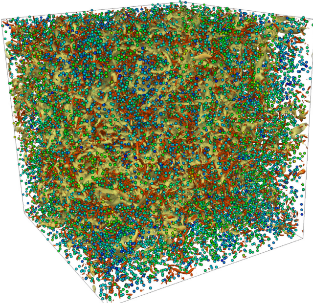
Fig. 4. Visualization of particle-laden decaying HIT. Particles are colored by their linear velocity (green-high and blue-low). Red denotes iso-surfaces of constant Q -criterion, while translucent yellow represents iso-surfaces of low pressure regions. Case 1024 simulated with IBM code, at time 1.25 T_0^e = 1 s. (For interpretation of the references to color in this figure legend, the reader is referred to the web version of this article.)
