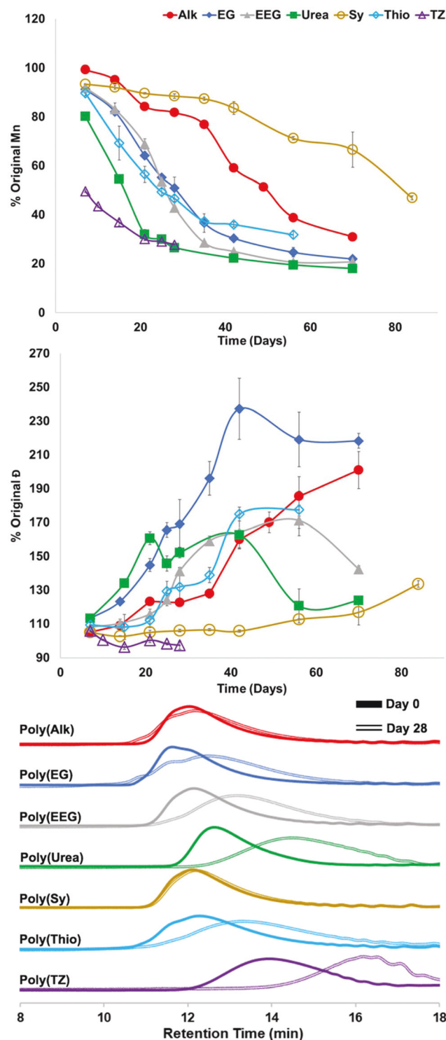
Fig. 5 Molecular weight ( M_n ) (top) and dispersity (middle) as a function of degradation time. Overlay of day 0 and day 28 size exclusion chromatography curves (bottom).
