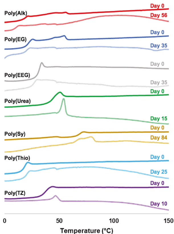
Fig. 2 Differential scanning calorimetry thermograms (endo up) of virgin and degraded polymers.
