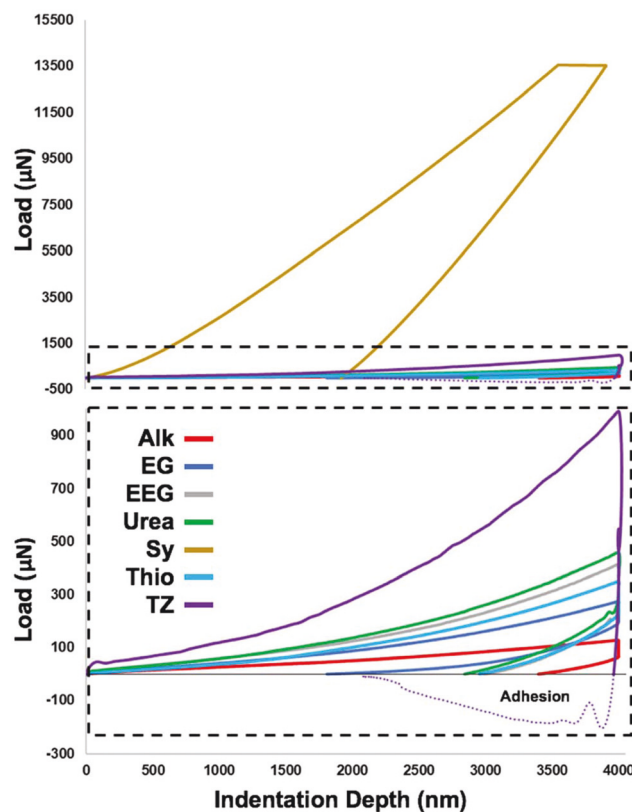
Fig. 3 Representative load-displacement curves for each polymer.
