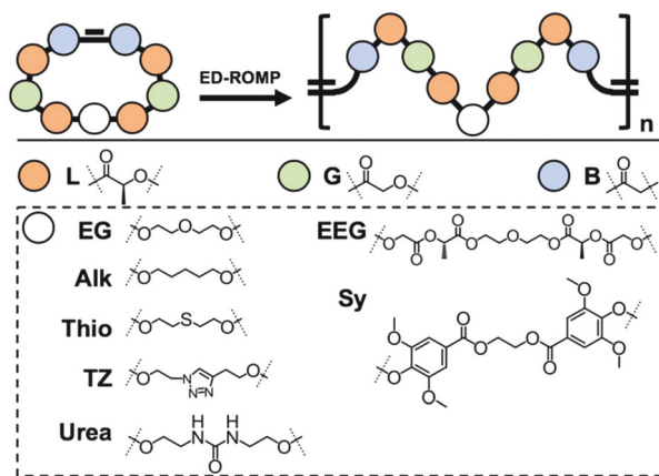
Fig. 1 Representation of sequence-controlled polymer with variable linker unit.
