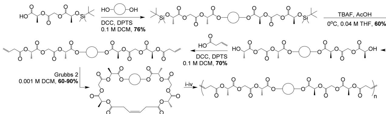
Scheme 1 Example synthetic scheme for the variable linker containing polymers. i (Alk, EG, EEG) – 1 mol% Grubbs 2, R.T., 0.7 M DCM, 4 h, 75%. ii (Urea, Sy) – 1 mol% Grubbs 2, 60 °C, 0.7 M THF, 4 h, 60–80%. iii (Thio) – 2.5 mol% Grubbs 2, 60 °C, 0.7 M THF, 4 h, 76%. iv (TZ) – 5 mol% Grubbs 2, 60 °C, 0.7 M THF, 4 h, 68%.
