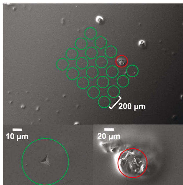
Fig. 4 Scanning electron microscopy images of Poly(Sy) at 50 \times (top), 1000 \times (bottom right) and 750 \times (bottom left) (bottom left shows a representative indentation).
