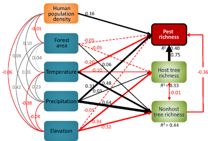
Fig. 3. Estimated structural equation model showing the effects of selected physical and human factors on pest diversity across conterminous United States (N = 2,098 counties). It also shows the effects of these factors on host and non-host tree diversity. Black lines indicate positive effects while the red lines indicate negative effects. The thickness of the lines indicates significance levels. Dashed lines indicate that the effects are non-significant (ns). R^2 represents the relative amount of variance explained for each dependent variable by the model. Values on the left are correlations among selected physical and social variables. The rest of the inserted values indicate the standard path coefficients. Standardized root mean square residual (SRMR) = 0.049, Goodness of Fit Index (GFI) = 0.965, root mean square error of approximation (RMSEA) = 0.221, McDonald Centrality = 0.979, Bentler Comparative Fit Index = 0.953, Akaike Information Criterion (AIC) = 377.121. Temperature and precipitation are annual means (see also Table S2). Note that the fit of models that include host and non-host biomass is rather poor, thus those models are not presented.
