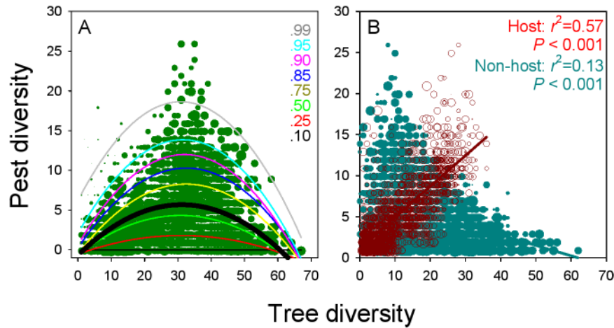
Fig. 1. The relationships between native tree species diversity (host plus non-host) and pest diversity across the conterminous United States (N = 2,098 counties; Symbol size reflects the relative forest area in each county). (A) Results based on second-order quantile regression for each quantile and polynomial regression for all data (i.e., data in all quantiles combined). The thinner hump-shaped regression curves were based on quantile thresholds of 0.1, 0.25, 0.5, 0.75, 0.85, 0.9, 0.95, and 0.99 from bottom to top, respectively. The corresponding equations and significance for each quantile are given in Table S1. The thicker black curve represents the second-order polynomial regression with all data [counties] considered, r^2 = 0.17 , P < 0.001 . In all cases, the pattern switched from positive to negative. (B) The opposite relationships between host tree species diversity and pest diversity, and between non-host tree diversity and pest diversity, across the conterminous United States.
