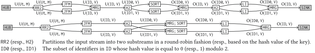
Figure 1. A transduction DAG that is equivalent to the one of Example 4.1 and allows data parallelism.
