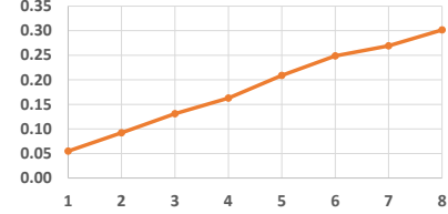
Figure 6. SMART HOMES - ENERGY PREDICTION: The horizontal (resp., vertical) axis shows the level of parallelization (resp., throughput in million tuples/sec).
