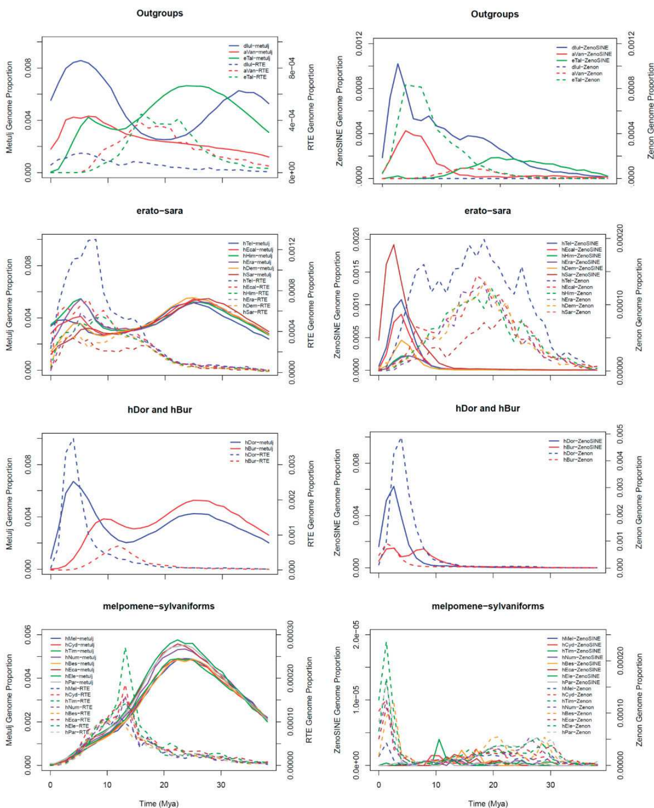
Fig. 4. —TE landscape plots for Metulj-RTE partners (left column) and ZenoSINE-Zenon partners (right column) in the four species divisions analyzed. The x axis depicts the estimated time of accumulation of the TE using the mutation rate described in the text. y axes depict genome proportions occupied by the TE for any given time on the x axis. Values for SINE-derived DNA are on the left axes and values for LINE-derived DNA are on the right axes.
