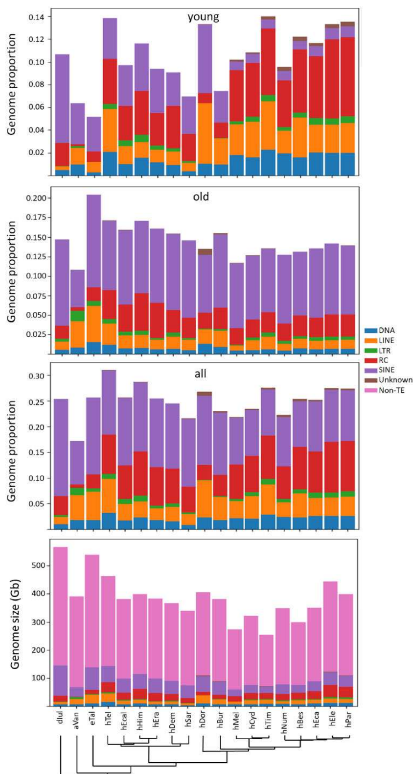
Fig. 2. —Stacked bar plots of TE proportions categorized as “old,” “young,” and “all” in each species examined. The combined plot at the bottom represents all data in the context of genome size. Species and their phylogenetic relationships (fig. 1) are depicted on the x axis. Abbreviations are as described in supplementary table 1, Supplementary Material online. Briefly, the first letter indicates genus, and the following three (or four) letters, except in the cases of Heliconius hecale and H. hecalesia , indicate species as listed in figure 1. Values on the y axis are genome proportions calculated as described in the text or total bp representation.
