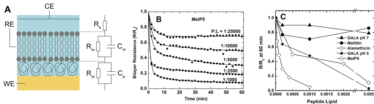
Figure 13. Electrochemical impedance spectroscopy. A. A polymer cushioned planar supported bilayer is adsorbed to the cleaned surface on a silicon crystal and the electrical properties are measured and modeled with an equivalent circuit. B. Resistance changes of a PC bilayer upon addition of the equilibrium pore former, MelP5. Note that the resistance does not recover as it would for a transient permeabilizing peptide. 66 C. Concentration dependence of the resistance drop for a variety of potent MPPs. Adapted with permission from ref 62. Copyright 2014 American Chemical Society.
