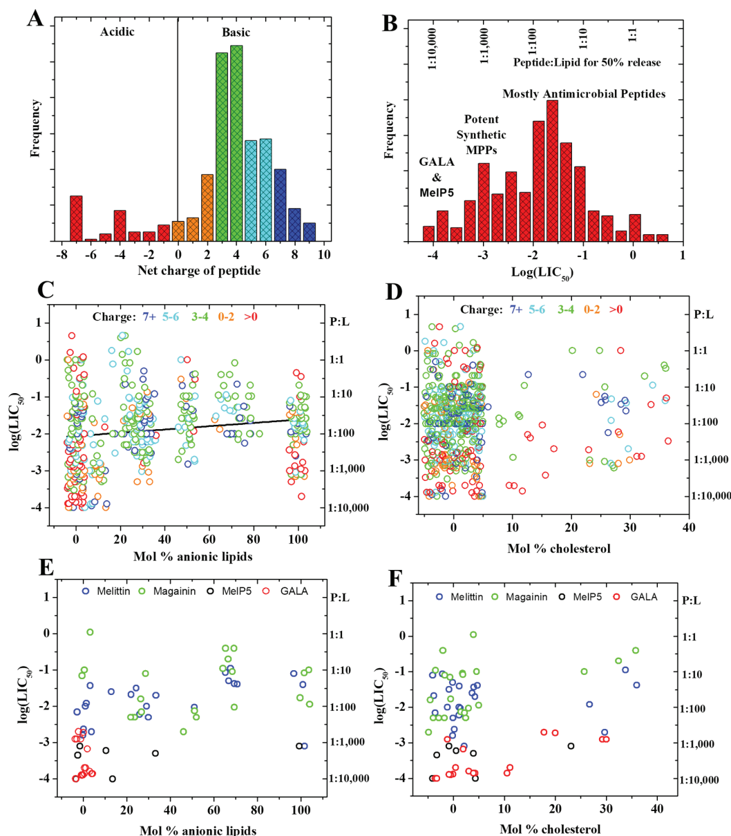
Figure 19. Meta-analysis of membrane permeabilizing peptides. A representative set of high quality published results was aggregated to show the range of behaviors observed for the permeabilization of synthetic vesicles by MPPs. A. Charge distribution in the data set. The colors used here are the same colors used in panels C and D. B. Distribution of the total peptide to lipid ratio required to release 50% of vesicle-entrapped contents, or LIC_{50} . C.: LIC_{50} plotted as a function of acidic lipid content (PG, PS, ganglioside, cardiolipin). The peptide charge states are shown by the color of the points, as shown in panel A. Random noise is added to the X-axis values to spread out the data points. D. LIC_{50} plotted as a function of cholesterol content. The peptide charge states are shown by the color of the points. E. LIC_{50} plotted as a function of acidic lipid content (PG, PS, ganglioside, cardiolipin) for a subset of well-studied peptides. F. LIC_{50} plotted as a function of cholesterol content for a subset of well-studied peptides.
