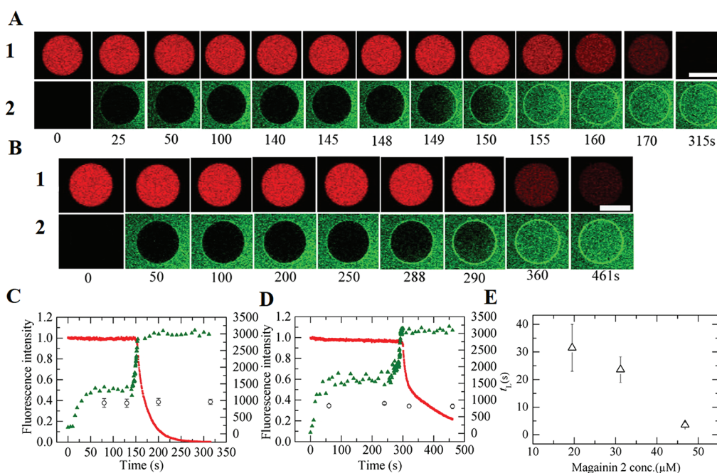
Figure 11. Peptide-induced permeabilization of GUVs. Membrane leakage of Alexa Fluor 647 hydrazide (AF647) and membrane permeabilization of carboxyfluorescein (CF)-labeled magainin 2 (CF-magainin 2) is visualized in single 40%DOPG/60%DOPC-GUVs. Panels A and B show confocal laser scanning microscopy (CLSM) images of (1) AF647 and (2) CF-magainin 2 in a single GUV treated with 31 \mu\text{M} CF-magainin 2/magainin 2 and 20 \mu\text{M} CF-magainin 2/magainin 2, respectively, at a certain time after of CF-magainin 2/magainin 2 addition to GUV denoted in seconds under each image. Panels C and D describe the time course of peptide-induced decrease in fluorescence intensity of AF647 in the GUV and increase in permeation of CF in the rim of GUV following the addition of CF-magainin 2/magainin 2. The solid red line corresponds to fluorescence intensity of AF647 inside the GUV while the green triangles correspond to the fluorescence intensity of CF-magainin 2 in the rim. The circles correspond to the fluorescence intensity of the outside vicinity of the GUV. FI = I(t)/I(0) , where I(t) and I(0) are the fluorescence intensity of AF647 inside the GUV at time t . Panel E refers to concentration dependent average lag time between the stochastic permeabilization of magainin 2 into the GUV and the leakage of dye from inside the GUV. These two phenomena can be studied by quantification of increase in the fluorescence intensities of the CF at the rim of the GUV and decrease in the fluorescence intensity of AF647 from inside the GUV. Adapted with permission from ref 358. Copyright 2015 American Chemical Society.
