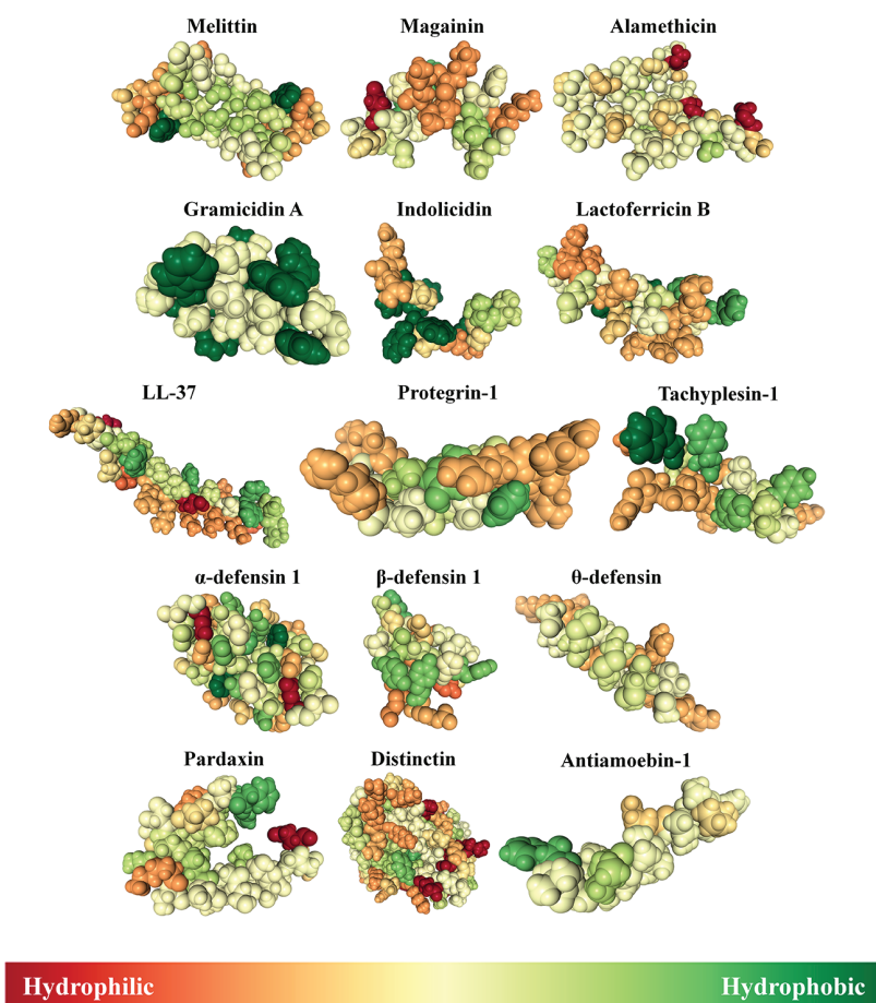
Figure 5. Amphipathic structures of membrane permeabilizing peptides. Space filling models for 15 peptides which are known membrane-permeabilizing peptides depicting hydrophobicity; no peptide here is depicted as singularly hydrophilic or hydrophobic, there are elements of both when considering MPPs.
