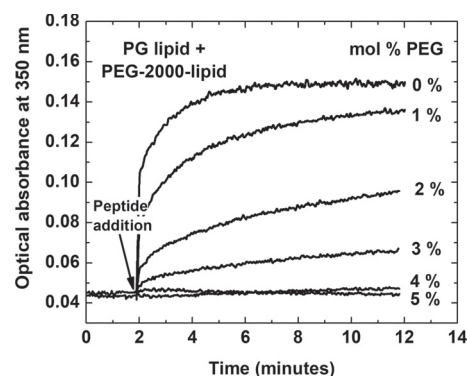
Figure 10. Cationic peptides rapidly aggregate anionic LUVs. Addition of the peptide *ARVA (RRGWALRLVLAY-amide) to POPG vesicles causes immediate and large scale aggregation of vesicles as shown by the increase in light scattering. Incorporation of PEG-2k-POPE lipids decreases aggregation dramatically, completely blocking it at 4–5 mol % PEG-lipids.
