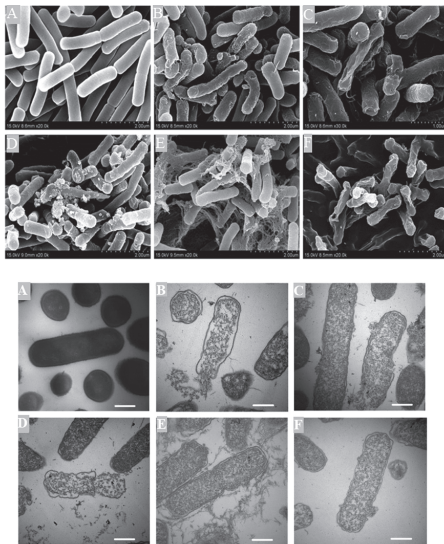
Figure 17. EM images of bacteria treated with AMPs. Top: SEM micrograph of E. coli ATCC 25922 (A) control; (B–E) synthetic centrosymmetric \alpha -helical AMP GG2, GG3, AA2, and AA3 treated; (F) MPP melittin treated. Bacterial cells were treated with 1 \times minimum bactericidal concentration (MBC) of peptide for 1 h. Adapted with permission from ref 529. Copyright 2015 Nature Publishing Group. Bottom: TEM micrographs of E. coli ATCC 25922. (A) Control; (B–E) synthetic centrosymmetric \alpha -helical AMP GG2, GG3, AA2, and AA3 treated; (F) MPP melittin treated. Bacterial cells were treated with 1 \times minimum bactericidal concentration (MBC) of peptide for 1 h. Scale bar = 500 nm. Adapted with permission from ref 529. Copyright 2015 Nature Publishing Group.
