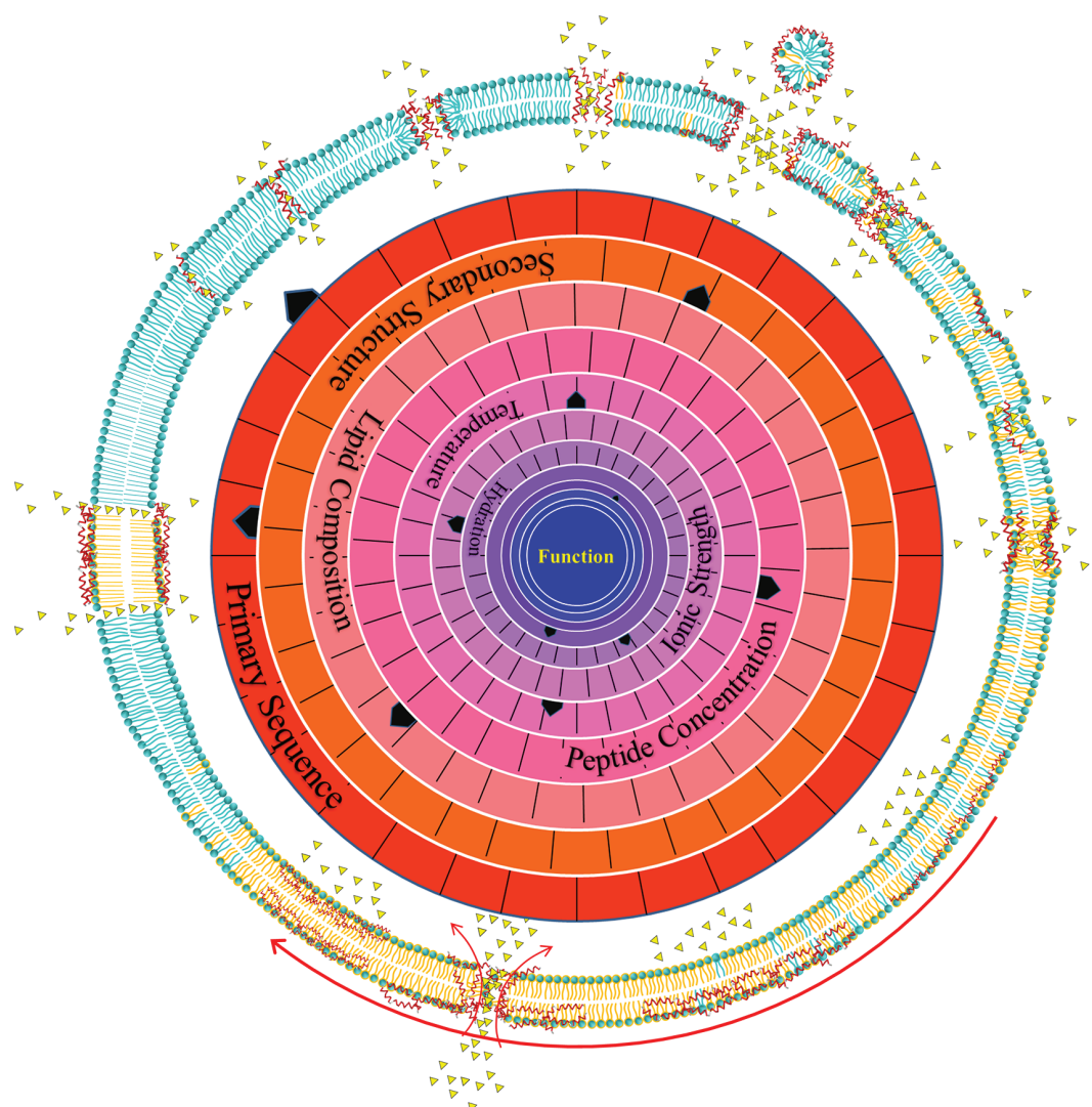
Figure 1. Mechanistic landscape of membrane permeabilizing peptides. The molecular mechanisms of membrane permeabilizing peptides have, for the most part, eluded atomic level description despite decades of intense study. As a result, their active structures and mechanisms are often drawn as cartoons like the imaginary snapshots arrayed in the cartoon bilayer above. Different colored lipids indicate changes in membrane composition, lipid tails, and headgroups. Curvy tails indicate fluid phase bilayers and straight tails indicate more ordered domains. In this review we describe how it might be useful to think of membrane permeabilizing peptides on a mechanistic landscape where molecular mechanism is not a fixed entity but instead depends on the sum of many experimental variables. The image in the center of the cartoon vesicle depicts concentric “dials”, one for each experimental variable (many are not explicitly shown). Each dial can be set to a particular “value” in the parameter space. The combinations of all of the settings give rise to a point on multidimensional mechanistic landscape.
