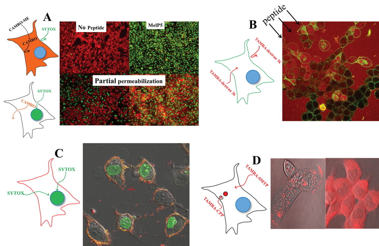
Figure 16. Examples of permeabilization of eukaryotic plasma membranes. A. Cells in culture were treated with calcein red orange acetoxymethyl ester, which freely crosses the cell and is activated by cellular esterases to become entrapped and membrane impermeant (red, upper left). At the same time SYTOX Green, a membrane impermeant DNA binding dye is added to the outside of the cells. Membrane permeabilization, as with MelP5 in the upper right, enables entry of SYTOX Green where it enters the nucleus and becomes fluorescent. B. In this confocal microscopy image, cell membranes are labeled green and a 3000 Da dextran labeled with TAMRA (red) is added outside the cells. Shortly after addition of a membrane permeabilizing peptide in the corner, the first cells exposed are permeabilized to the dextran and they show osmotic swelling. The cells in the opposite corner have not yet been affected by peptide. C. Cell membranes are labeled red and cells are incubated with external SYTOX Green. A low concentration of the Ebola Virus delta peptide, a viroporin, 136 was added 10 min prior to taking this image. Here cells have been permeabilized to SYTOX Green, which stains the nuclei, but massive water influx and osmotic lysis are not occurring, evidenced by the lack of swelling or cell rounding at this time. D. TAMRA-labeled cell penetrating peptide (Arg 9 -TAMRA) and a spontaneous membrane translocating peptide TP2-TAMRA 38 are incubated with cells at a low concentration of \sim 1 \mu\text{M} . The CPP gets untaken into endosomes, but cannot escape into the cytosol, in this case, because its concentration is too low to disrupt the membrane. The translocating peptide spontaneously crosses the plasma membrane and enters the cytosol. We thank Kalina Hristova for generous access to her confocal microscope.
