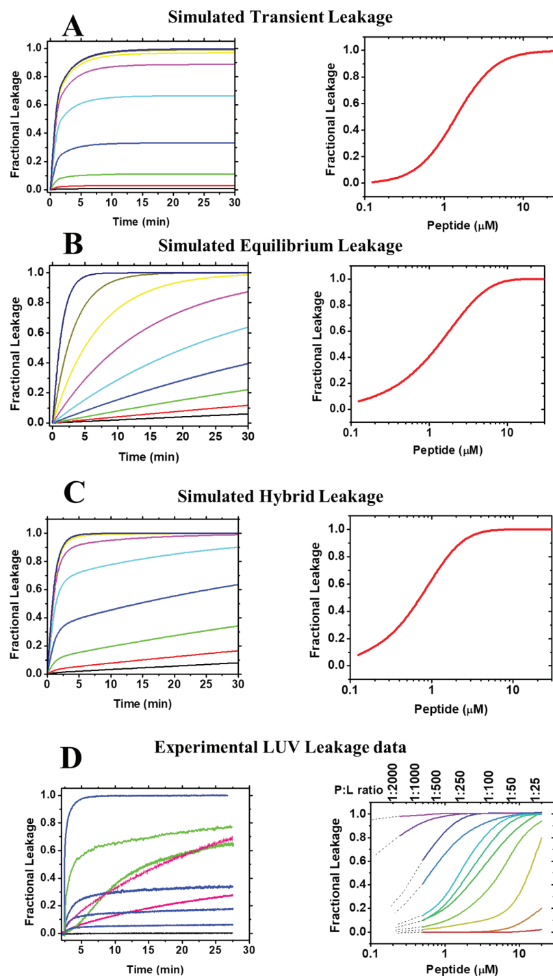
Figure 20. Experimental and simulated permeabilization of LUVs. We simulate vesicle leakage using simple numerical models. A. Transient leakage has a constant exponential rise toward a final value that itself depends on the P:L in the experiment. Many leakage experiments have behavior like this. The exponential rise assumes that the fraction of remaining entrapped contents released per unit time is constant. The plot on the right shows potency profile in a semilog plot. B. Simple equilibrium leakage model assumes an exponential rise toward 100% release where the rate (the fraction of remaining entrapped contents released per unit time) is a function of peptide concentration. This behavior is rarely observed. The plots on the right shows potency profile at 30 min in a semilog plot. C. Hybrid leakage, assumes that there is a major component of transient leakage, followed by a low level steady equilibrium release. Many peptides have this behavior. D. Real experimental leakage curves for various MPPs taken from the authors' manuscripts. Real curves like all three of these simulations are seen in this set. The plots on the right shows various potent curves taken from the authors' manuscripts. They range from high potency MPPs (e.g., alamethicin) that release \sim 100\% of contents at P:L = 1:2000 to some AMPs or analogs that release almost nothing at P:L of 1:10. Peptides, lipid compositions, and other details vary in these curves.
