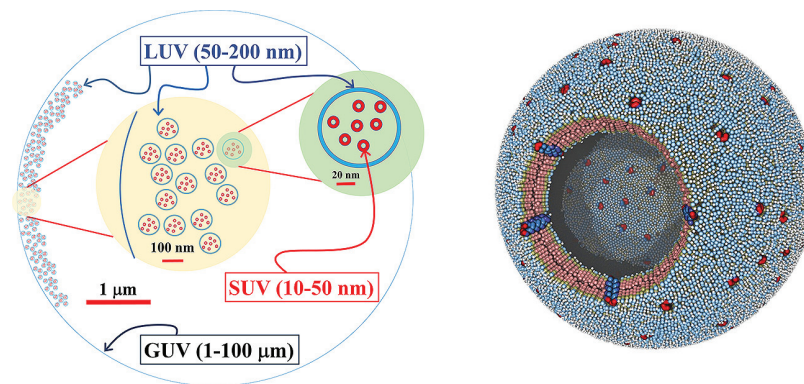
Figure 6. Realistic cartoons of lipid vesicles. In this cartoon, small (SUV), large (LUV), and giant (GUV) unilamellar vesicles are drawn roughly to scale in three different magnifications. Even the membrane thickness is drawn to scale in each magnifications. On the right is a simulation of a vesicle of 34 nm diameter, containing \sim 40\,000 lipids. Image courtesy of Andrew Jewett at www.moltemplate.org .
