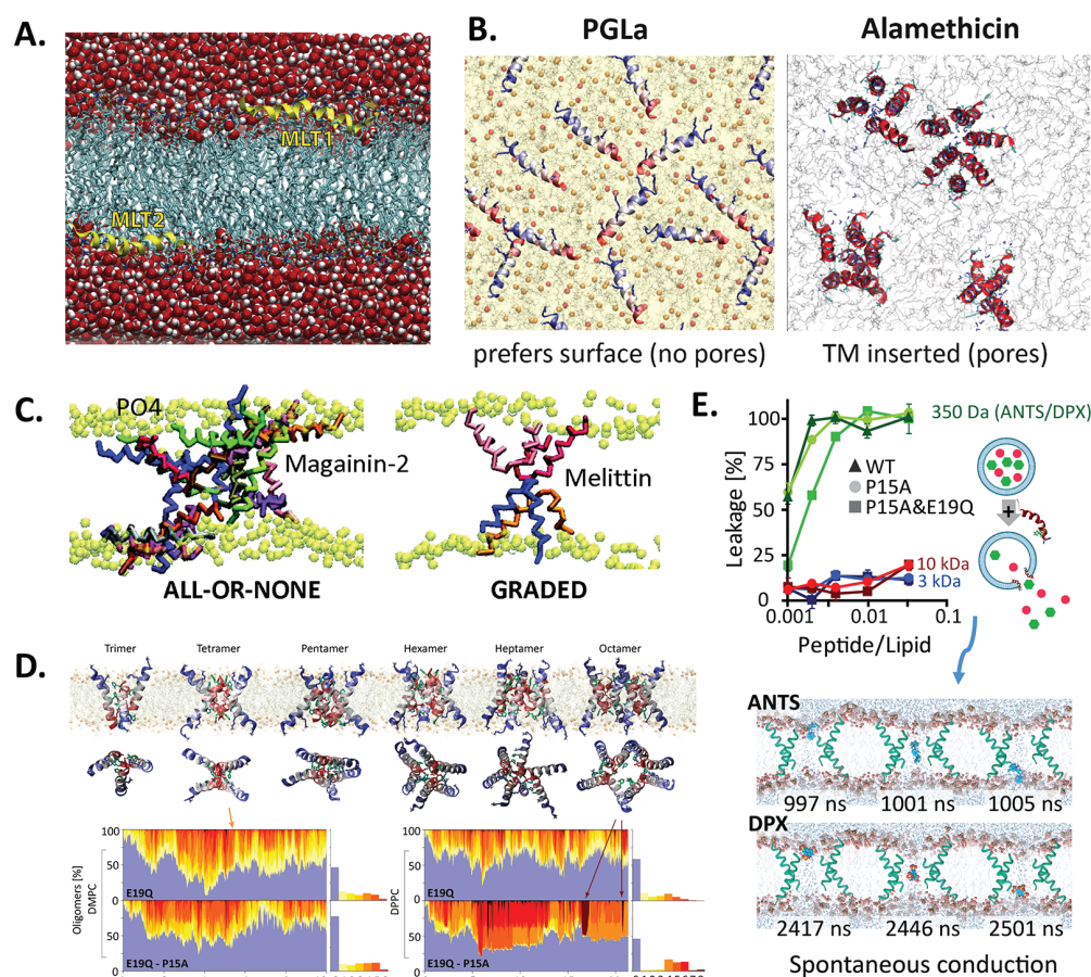
Figure 15. Molecular dynamics simulations of MPPs show binding and structure formation on and in bilayers. (A) A simulation of melittin monomer binding over 17 \mu s shows that the peptide settles at a depth near the glycerol groups, which notably is consistent with X-ray diffraction results. Adapted with permission from ref 429. Copyright 2013 Elsevier, Inc. (B) Two different behaviors of multiple peptides binding to a bilayer are shown here. The interfacial S state is preferred by PGLa while a transmembrane configuration is preferred by alamethicin, a known potent pore former. Adapted with permission from ref 405. Copyright 2018 American Chemical Society. (C) Transmembrane structures of an all-or-none and graded peptide. Melittin peptides are in a U-shape that blocks water passage while magainin-2 allows water through more easily. These simulations indicate how all-or-none and graded mechanisms can be structurally different. Adapted with permission from ref 432. Copyright 2012 American Chemical Society. (D) Permeabilization is complex, as shown with the example of maculatin. The peptide does not form just one structure on a bilayer; it forms a variety of structures that assemble and disassemble over time for both DMPC and DPPC bilayers (bottom). However, it should be noted that most peptides are in the surface bound state (S). (E) Unbiased dye-conductance simulations show that P15A-E19Q, a maculatin double mutant that is thermally stable, forms lesions just large enough to allow ANTS and DPX through (bottom). Importantly, this finding was validated with experimental ANTS/DPX and dextran release assays (top). Panels D and E adapted with permission from ref 411. Copyright 2016 Springer Nature Limited (CC) https://creativecommons.org/licenses/by/4.0/legalcode .
