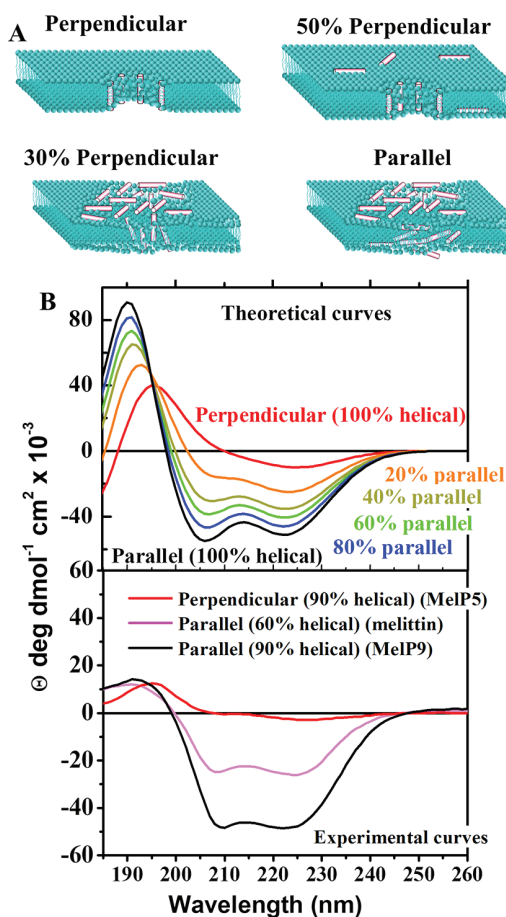
Figure 14. Oriented circular dichroism. In OCD, oriented multibilayers stacks containing a peptide that has mostly \alpha -helical secondary structure are prepared on a quartz disk and hydrated through the vapor phase. Circular dichroism is measured with the bilayer plane oriented perpendicular to the beam axis. A. Bilayers with imaginary helical MPPs that have axes perpendicular or parallel to the bilayer normal, or a combination of the two. B. Theoretical spectra for perpendicular (transmembrane) and parallel (surface-oriented) \alpha -helices are shown, along with linear combinations of the two. 194 These data are scaled to represent residue contributions assuming 100% helicity. C. Real experimental OCD data 59 for melittin, which is parallel to the bilayer and has a helicity of \sim 60\% , and two gain of function analogs, MelP5, which is perpendicular to the bilayer and has 90% helix, and MelP9, which is parallel to the bilayer and has 90% helix. Adapted with permission from ref 181. Copyright 2018 American Chemical Society.
