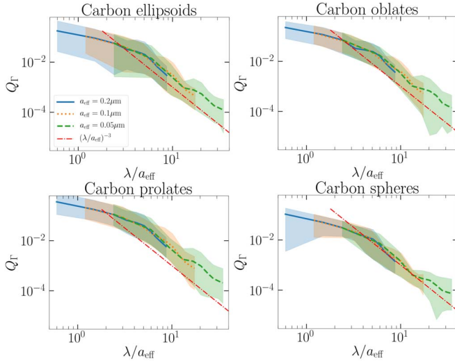
Figure 22. Same as Figure 20, but for carbonaceous shapes.
