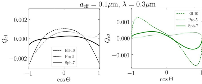
Figure 7. Same RAT components as Figure 4, but for \lambda = 0.3 \mu\text{m} , with grains exhibiting mostly left-handed helicity. The prolate grain 5 transitions to right-handed helicity when the major principal axis is nearly parallel to the incident radiation direction.
