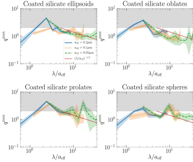
Figure 16. Same as Figure 15, but for coated silicates.
