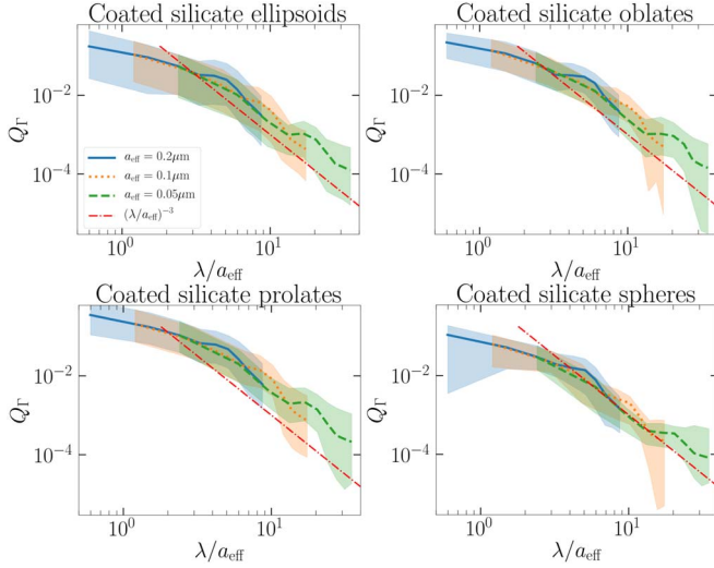
Figure 21. Same as Figure 20, but for coated silicates.
