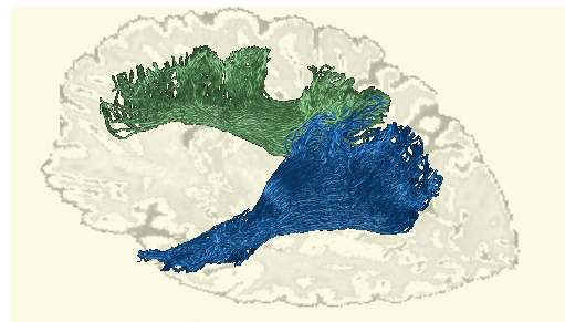
Candidate connectome
