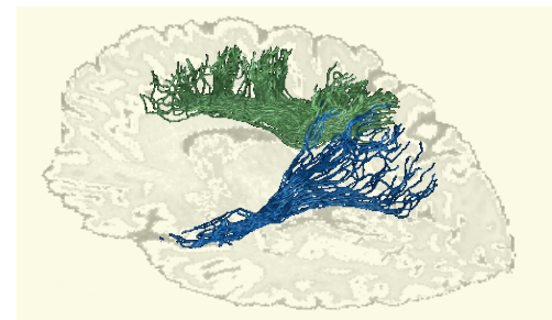
Pruned connectome
