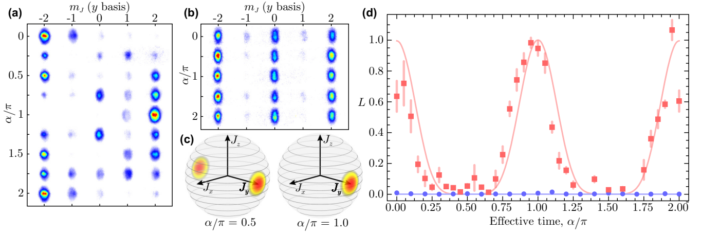
FIG. 4. Squeezing of the artificial spin. Absorption images of the y-basis spin projection as a function of the effective squeezing time \alpha when starting in (a) |\theta = \pi/2, \phi = -\pi/2\rangle_{\text{CSS}} and (b) |J = 2, m_J = 0\rangle_z . (c) Density distributions for initial state |\theta = \pi/2, \phi = -\pi/2\rangle_{\text{CSS}} shown at effective times \alpha/\pi = 0.5 (left) and \alpha/\pi = 1.0 (right). (d) Spin length L versus the effective squeezing time \alpha . The red squares and simulation line are for initial state |\theta = \pi/2, \phi = -\pi/2\rangle_{\text{CSS}} , and the blue dots and simulation line are for |J = 2, m_J = 0\rangle_z . All error bars are one standard error of the mean.
