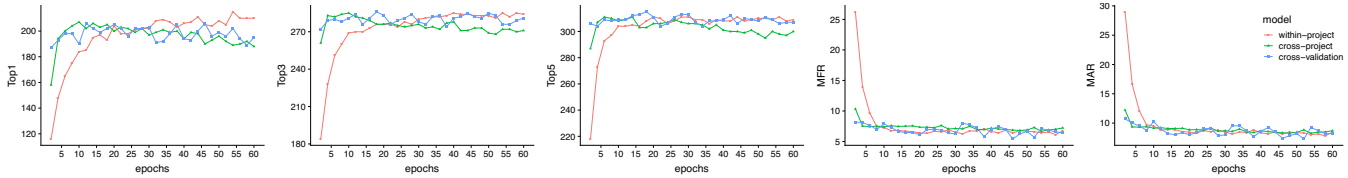
Figure 9: Impacts of different epochs for within-project, cross-project and cross-validation predictions
