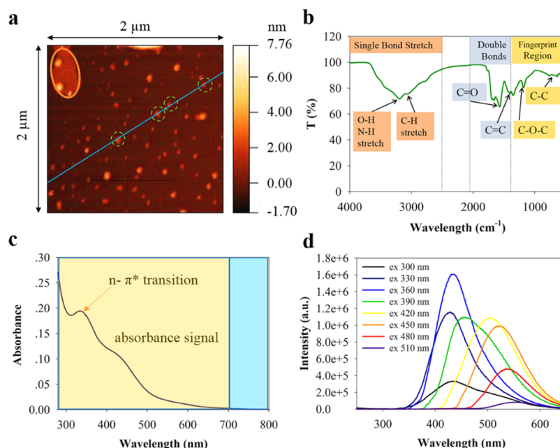
Figure 2. Characterization of the CNDs by different techniques: (a) AFM topography image, (b) FTIR spectra, (c) UV-vis absorption spectra, and (d) fluorescence emission spectra.
