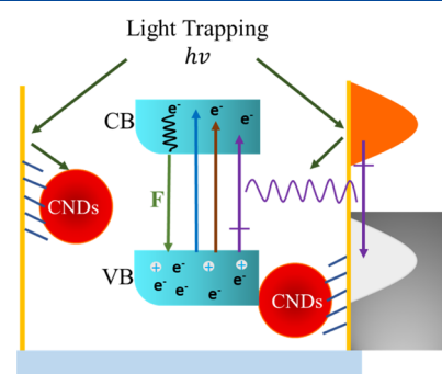
Figure 6. Schematic diagram illustrating the proposed process of fluorescence enhancement of CNDs because of SPR generation and energy transfer in a gold nanoslit.
