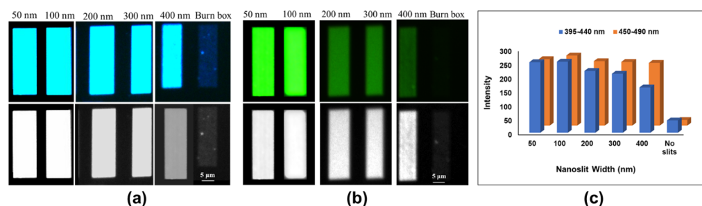
Figure 3. Fluorescence images of different width nanoslit arrays with the Axio Z2M microscope. (a) Upper panel shows the images taken using a 395–440 nm filter light source, and lower panel shows the same fluorescent images when converted to gray-scale images; (b) fluorescence images (upper panel) taken using a 450–490 nm filter and converted gray-scale images (lower panel); and (c) graphic plot showing the fluorescence intensity measured with different filters corresponding to different nanoslit width arrays.
