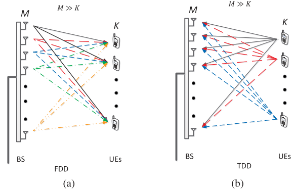
Fig. 1. (a) FDD massive MIMO requires M orthogonal pilots, (b) TDD massive MIMO requires K orthogonal pilots.
