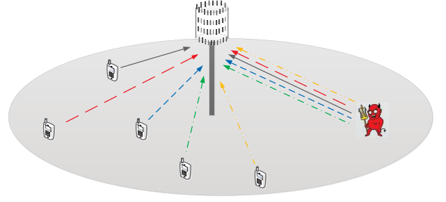
Fig. 2. Pilot contamination attack model in a multi-user massive MIMO system.
