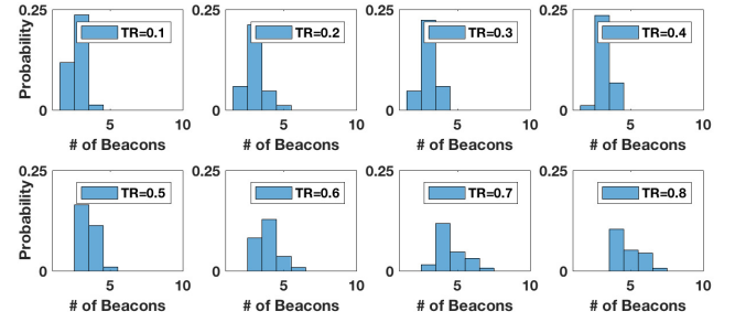
Figure 22: Alignment efficiency: EAR can finish the alignment within 7 beacon periods (corresponding to 700ms) even in the worst case ( TR=0.8 ).
