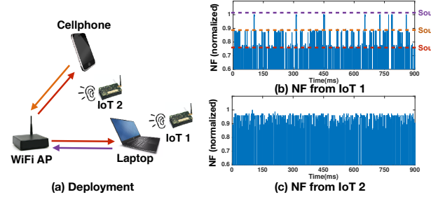
Figure 4: Some IoT devices (i.e., IoT 1) can distinguish signal sources via NF while the others (i.e., IoT 2) cannot.
