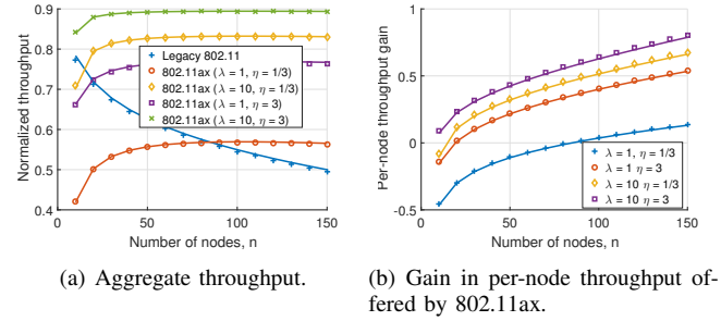
Fig. 3: Aggregate MAC-layer throughput.
