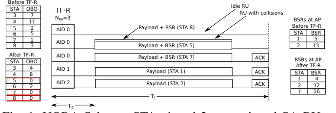
Fig. 1: UORA Scheme. STAs 1 and 2 are assigned SA RUs, while other STAs contend for transmissions on the three RA RUs. STAs 5, 7 and 8 decrement their OBOs to zero and transmit on randomly selected RUs leading to a collision on the second RA RU and successful transmission on the third RA RU; the first RA RU remains idle.
