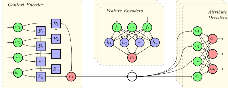
Fig. 4. The model architecture encodes a context window as a sequence of tokens w_1 to w_n using a BiLSTM which is represented with forward and backward cells. The encoding is then used in combination with our other feature sets for decoding. A separate decoder is used for each speaker attribute.
