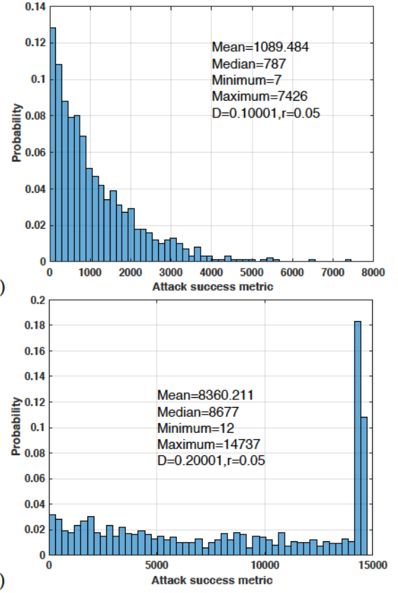
Fig. 7: Histogram of simulation results in which (a) the cloud is about twice faster than the attacker, and (b) the cloud is about four times faster than the attacker. The x-axis shows the attack success metric, the number of vertices the attacker tried until reaching the target. The y-axis shows the sample probability of the attack success metric.
