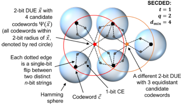
Fig. 1: Two-dimensional illustration of candidate codewords for 2-bit DUEs in the n -dimensional Hamming space of a binary SECDED code.
