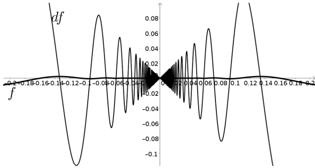
Fig. 2.4. The function f(x) = x^3 \sin(\frac{1}{x}) and its derivative.
