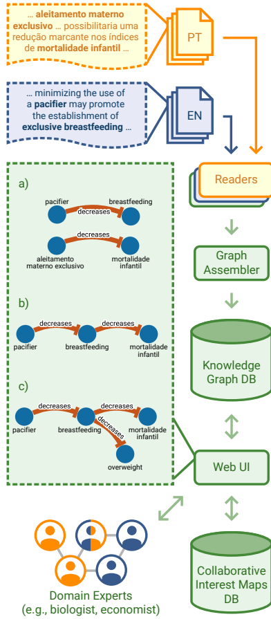
Figure 1: System architecture and example. Causal relations from sentences about breastfeeding in English (Mastrup et al., 2014) and Portuguese (Cavalcanti et al., 2015) are extracted and used by domain experts to collaboratively build a shared causal model of the task of interest, called an interest map, through a web UI. (a) A user searches for causes of breastfeeding and effects of aleitamento materno exclusivo (exclusive breastfeeding), and adds two interesting links to a shared interest map. (b) A second user merges aleitamento materno exclusivo and breastfeeding . (c) A third user adds an additional link (to overweight ) from a new search to the shared interest map. The constructed interest maps are stored in a separate database, where they can be edited in real-time by collaborators.
