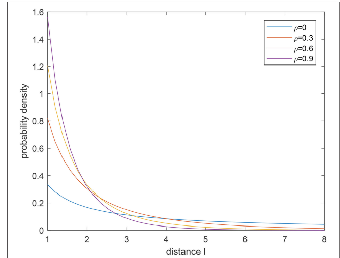
FIGURE 3 | Probability density for tempered Lévy distribution with \mu = 1 for different \rho .
