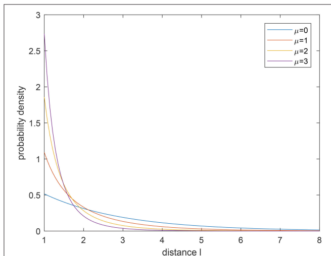
FIGURE 2 | Probability density for tempered Lévy distribution with \rho = 0.5 for different \mu .
