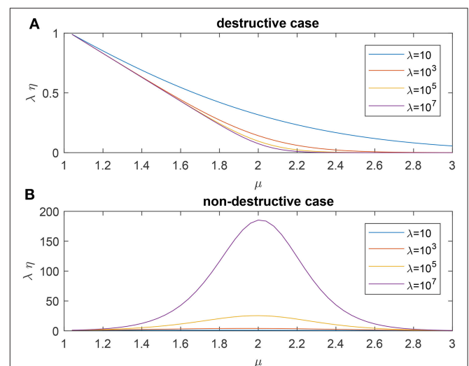
FIGURE 1 | Searching efficiency of standard Lévy flight for different mean free path \lambda : (A) the destructive case, (B) the nondestructive case.
