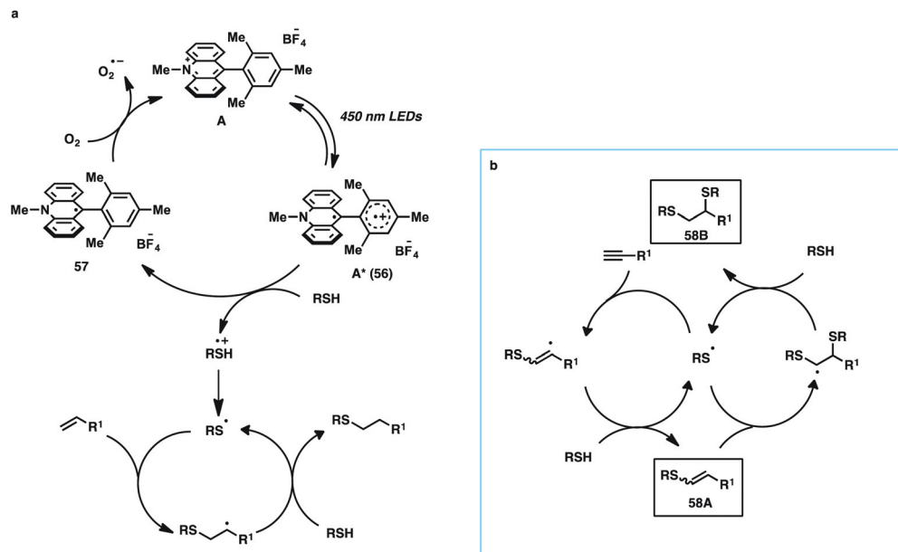
Scheme 6 Proposed mechanism.
