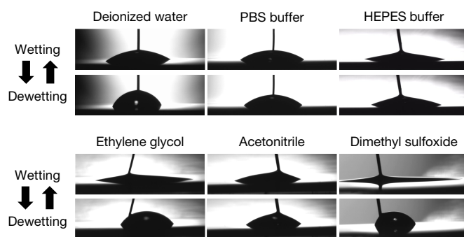
Fig. 4 | The proposed electrode wetting confirmed for a variety of liquids on bare silicon. Deionized water (Fig. 1) is included as a reference. DTAB was used for all, with different concentrations as described in the Methods. For PBS and HEPES, contact-angle changes of approximately 9^\circ and 6^\circ were obtained, respectively, using \pm 5 V. For ethylene glycol, acetonitrile and DMSO, changes of approximately 40^\circ , 15^\circ and 60^\circ were obtained, respectively, using \pm 3 V.
