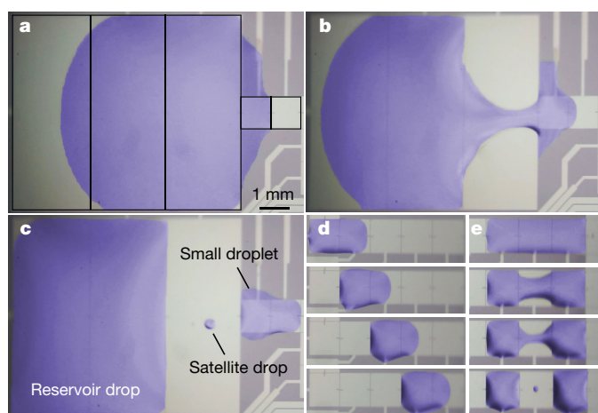
Fig. 3 | Droplet generation, transportation and splitting realized by the proposed electrode wetting. Water droplets are operated in air on a silicon device with no cover plate, using \pm 2.5 V (or 0 V and 5 V). Images were captured from Supplementary Video 4 and enhanced by colouring the liquid portions. a–c , Sequential images of a small (about 0.2 \mu\text{l} ) droplet generated from a reservoir droplet (about 3 \mu\text{l} ). a , The black lines were added to indicate the large electrodes underneath the reservoir. b , Dewetting the third reservoir electrode from left results in necking of the reservoir droplet. c , A droplet is generated on the two small electrodes to the right of the reservoir. d, e , Sets of four sequential images showing droplet transportation ( d ) and splitting ( e ). Along with droplet generation (panels a to c ) and merging (not shown), they establish the basic operations of digital microfluidics.
